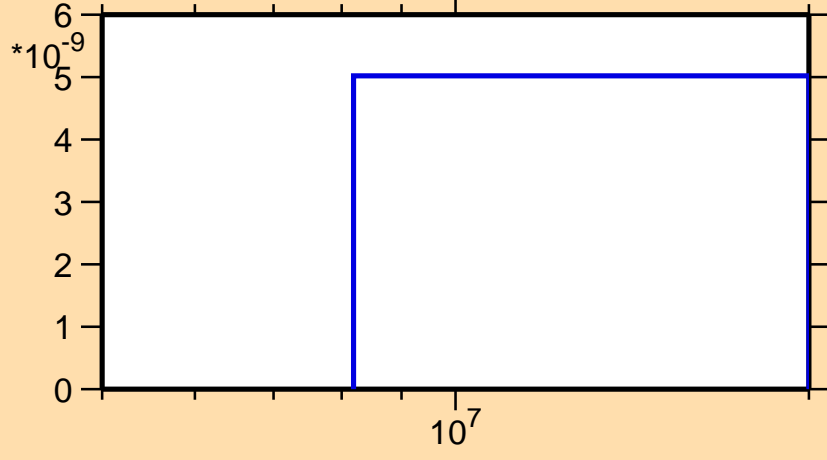
\sigma vs. E for ^{207}\text{Bi}(n,nt)
