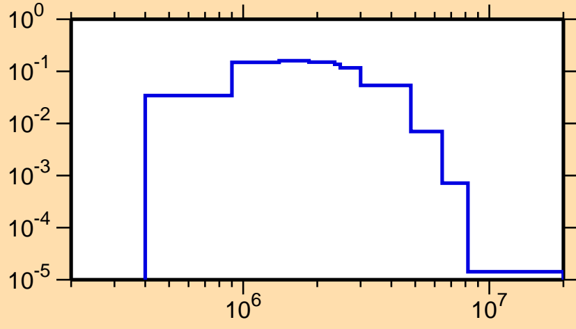
\sigma vs. E for ^{208}\text{Bi}(n,n_4)
