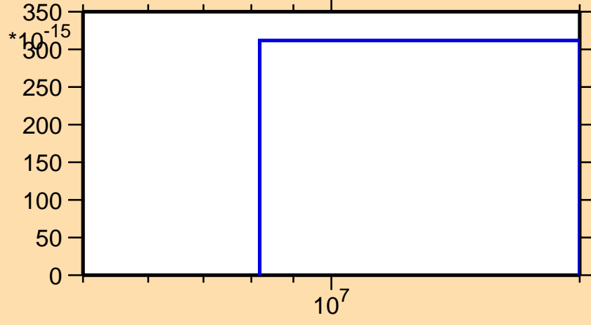
\sigma vs. E for ^{208}\text{Bi}(n,p\alpha)
