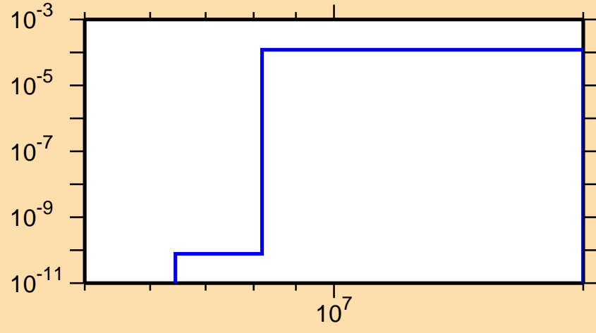
\sigma vs. E for ^{208}\text{Bi}(n,t)
