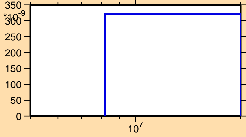
\sigma vs. E for ^{208}\text{Bi}(n,\text{nd})
