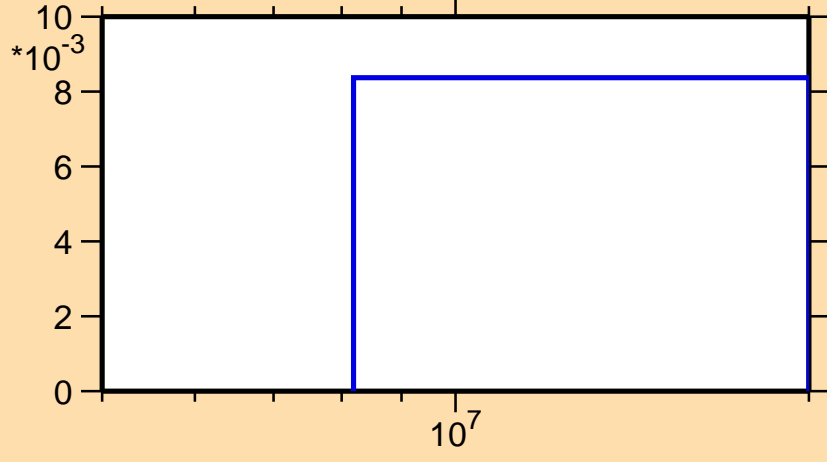
\sigma vs. E for ^{208}\text{Bi}(n,3n)
