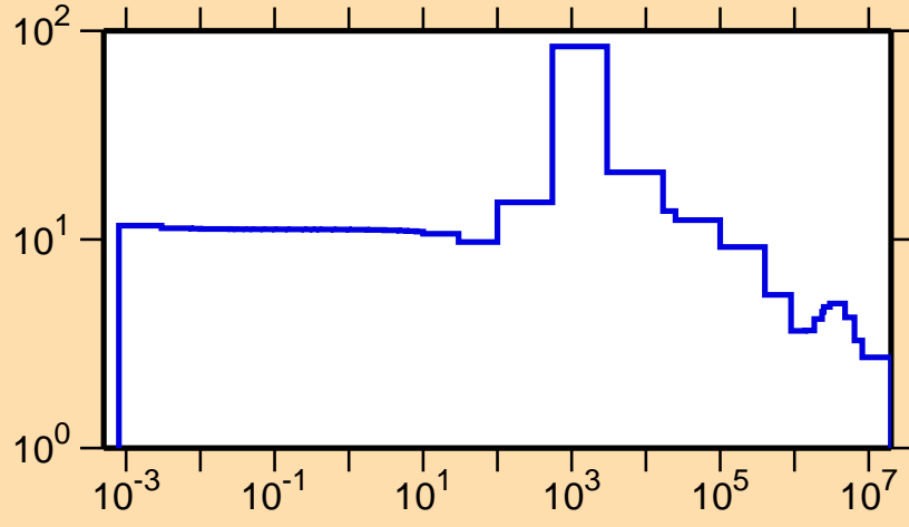
\sigma vs. E for ^{208}\text{Bi}(n,\text{el.})
