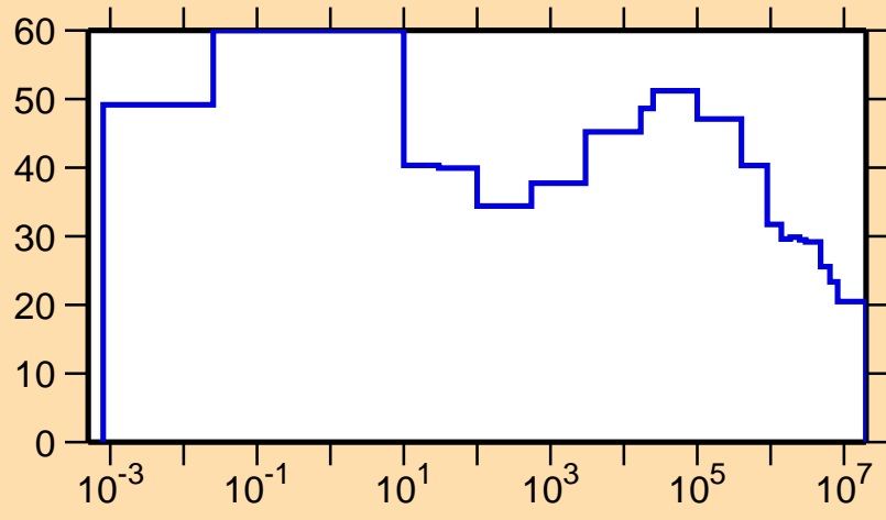
\Delta\sigma/\sigma vs. E for ^{208}\text{Bi}(n,p)
