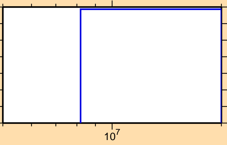
\sigma vs. E for ^{208}\text{Bi}(n,2np)
