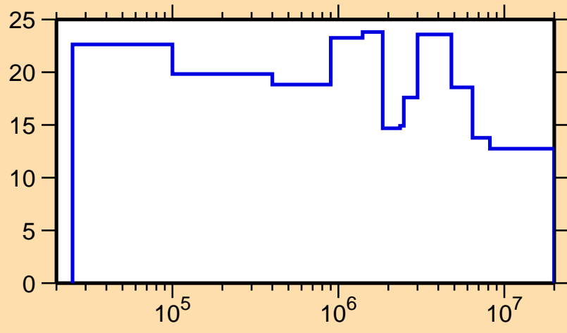
\Delta\sigma/\sigma vs. E for ^{208}\text{Bi}(n,n_1)
