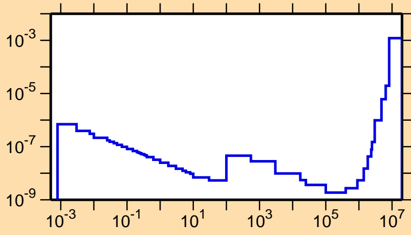
\sigma vs. E for ^{208}\text{Bi}(n,\alpha)
