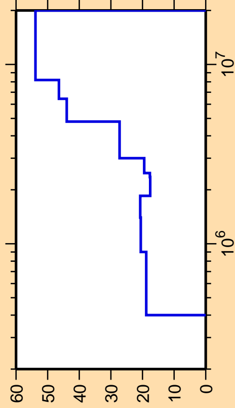
\Delta\sigma/\sigma vs. E for ^{208}\text{Bi}(n,n_4)
