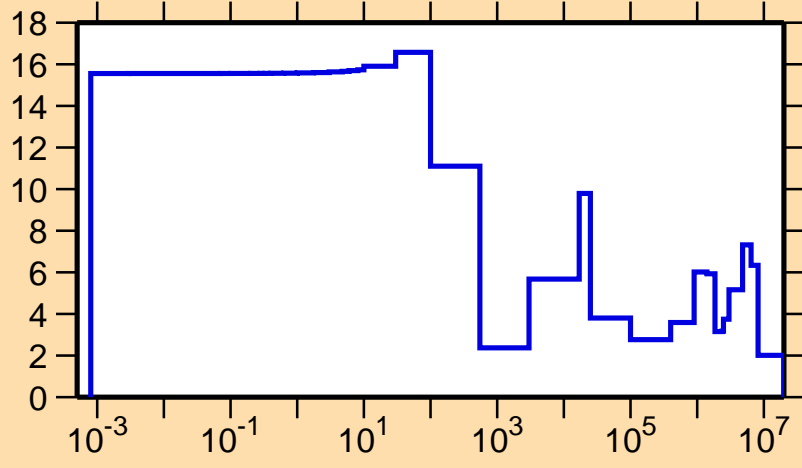
\Delta\sigma/\sigma vs. E for ^{208}\text{Bi}(n,\text{el.})
