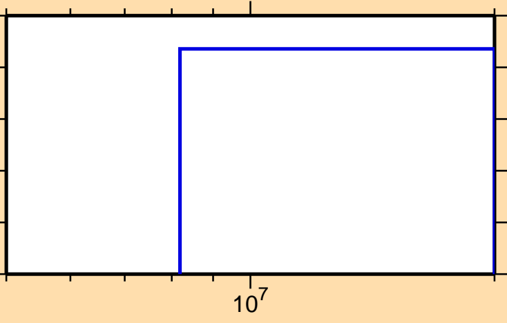
\sigma vs. E for ^{208}\text{Bi}(n,2n\alpha)
