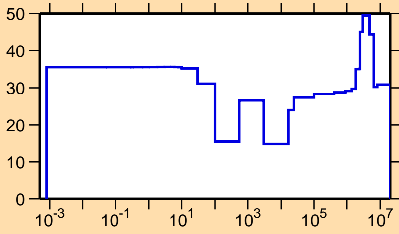
\Delta\sigma/\sigma vs. E for ^{208}\text{Bi}(n,\gamma)
