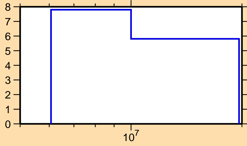
\Delta\sigma/\sigma vs. E for ^{209}\text{Bi}(n,2n)
