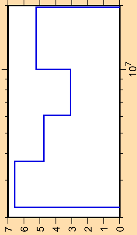
\Delta\sigma/\sigma vs. E for ^{209}\text{Bi}(n,n\text{cont.})
