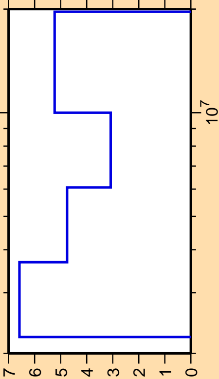
\Delta\sigma/\sigma vs. E for ^{209}\text{Bi}(n,n\text{cont.})
