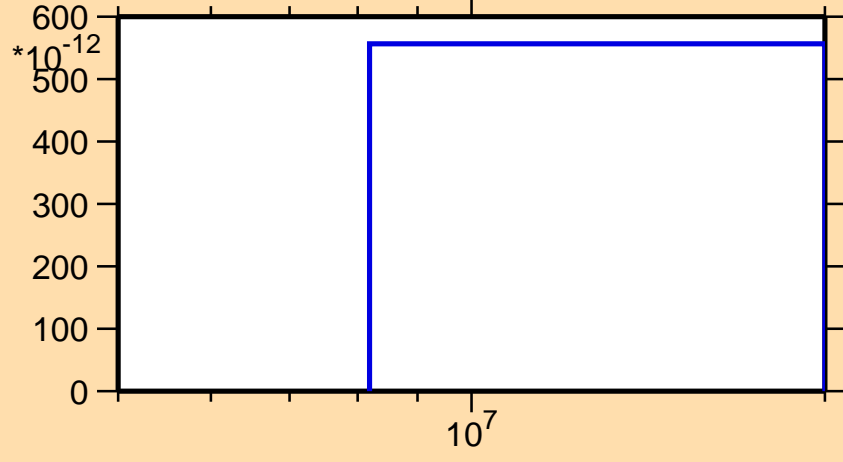
\sigma vs. E for ^{209}\text{Bi}(n,2n\alpha)
