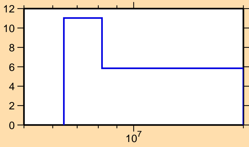
\Delta\sigma/\sigma vs. E for ^{209}\text{Bi}(n,2n)
