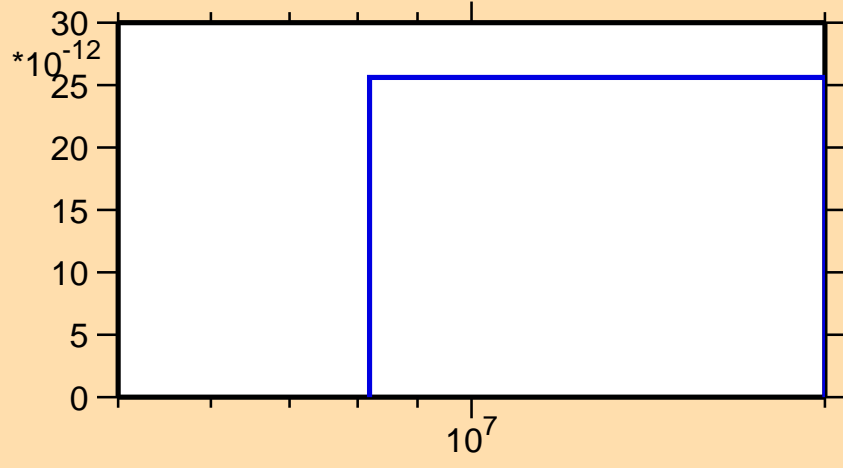
\sigma vs. E for ^{209}\text{Bi}(n,\text{He3})
