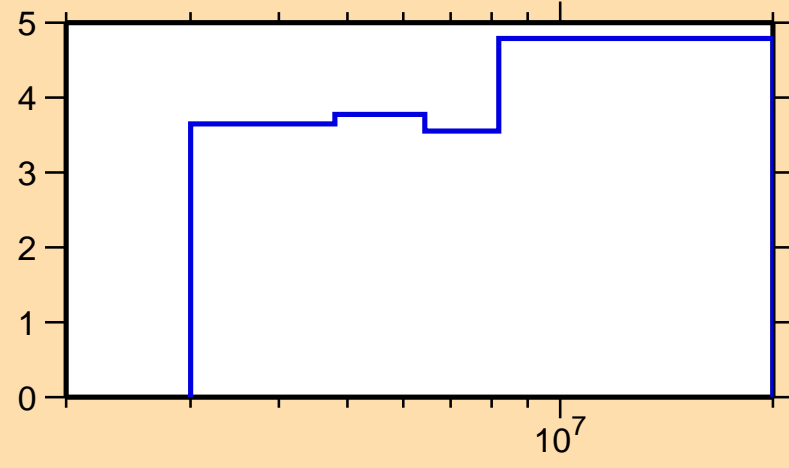
\Delta\sigma/\sigma vs. E for ^{209}\text{Bi}(n,n\text{nonel.})
