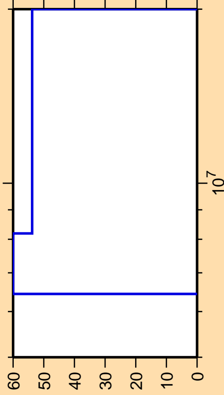
\Delta\sigma/\sigma vs. E for ^{209}\text{Bi}(n,\alpha)
