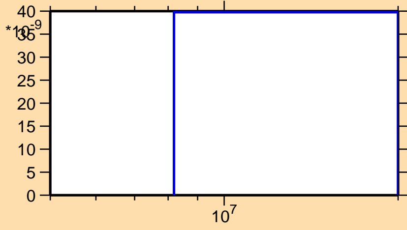
\sigma vs. E for ^{209}\text{Bi}(n,2np)
