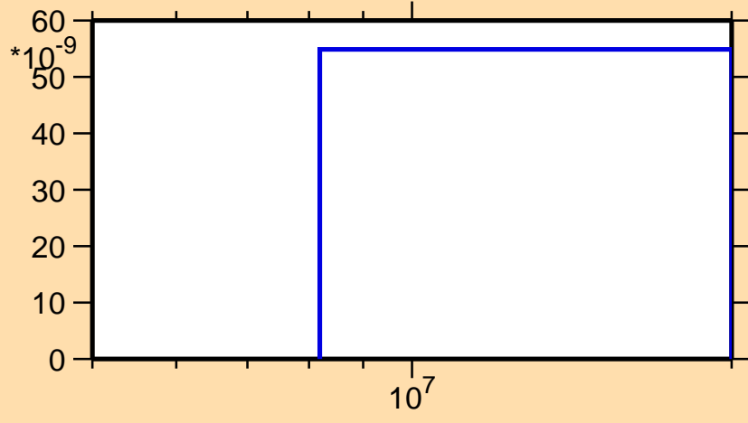
\sigma vs. E for ^{209}\text{Bi}(n,\text{nd})
