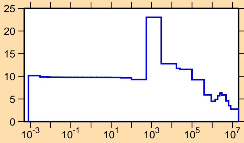
\sigma vs. E for ^{209}\text{Bi}(n,\text{el.})
