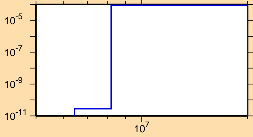
\sigma vs. E for ^{209}\text{Bi}(n,t)
