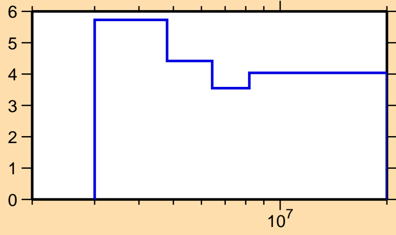
\Delta\sigma/\sigma vs. E for ^{209}\text{Bi}(n,n\text{cont.})
