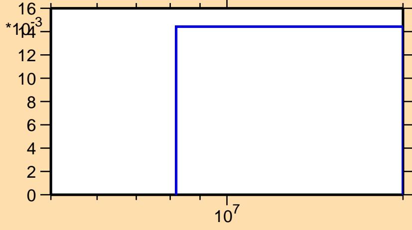
\sigma vs. E for ^{209}\text{Bi}(n,3n)
