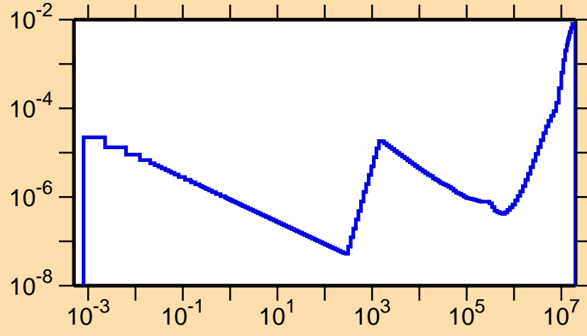
\sigma vs. E for ^{210}\text{Bi}(n,\alpha)
