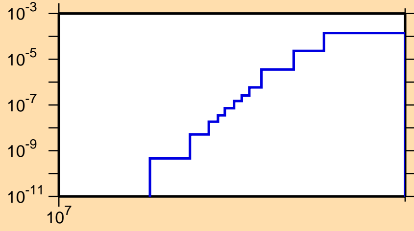
\sigma vs. E for ^{210}\text{Bi}(n,nt)
