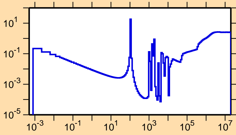
\sigma vs. E for ^{210}\text{Bi}(n,\text{nonel.})
