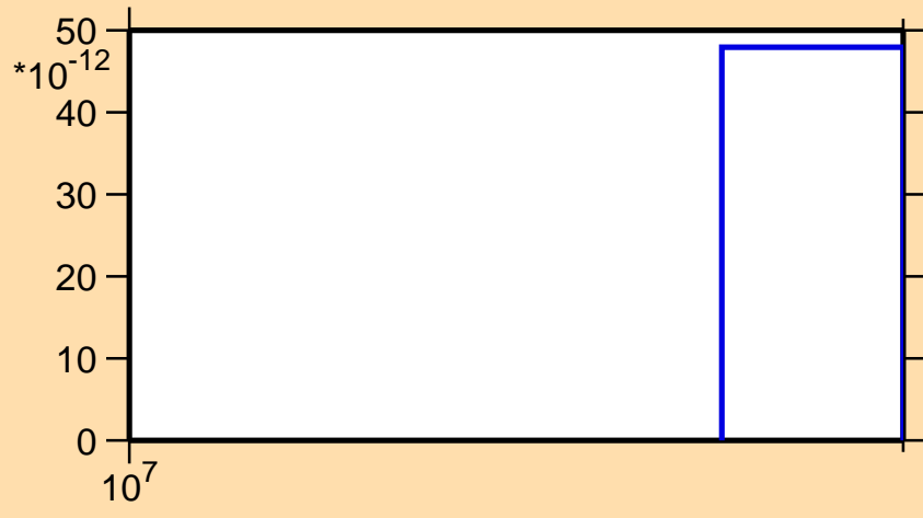
\sigma vs. E for ^{210}\text{Bi}(n,p\alpha)
