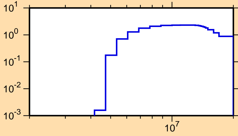
\sigma vs. E for ^{210}\text{Bi}(n,2n)
