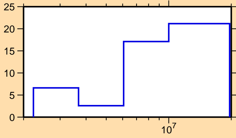
\Delta\sigma/\sigma vs. E for ^{210}\text{Bi}(n,ncont.)
