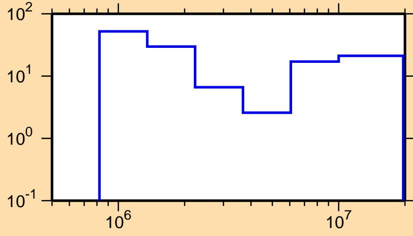
\Delta\sigma/\sigma vs. E for ^{210}\text{Bi}(n,n\text{cont.})
