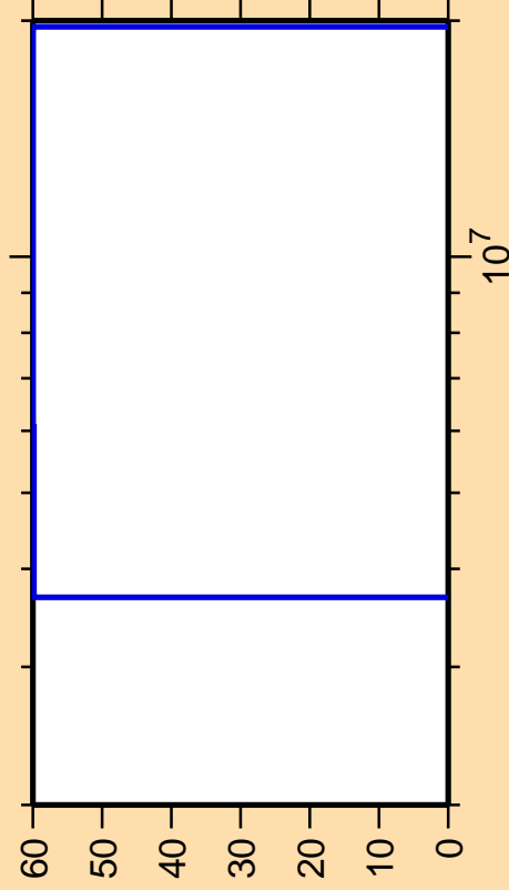
\Delta\sigma/\sigma vs. E for ^{210}\text{Bi}(n,t)
