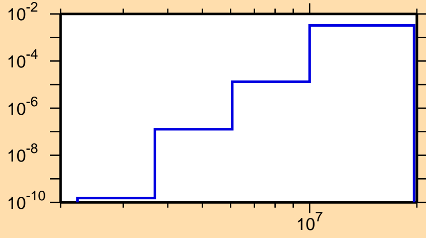
\sigma vs. E for ^{210}\text{Bi}(n,p)
