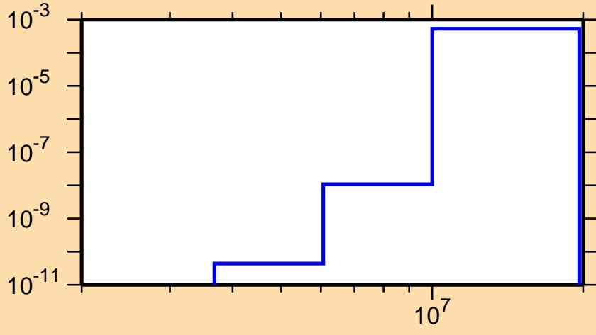
\sigma vs. E for ^{210}\text{Bi}(n,t)
