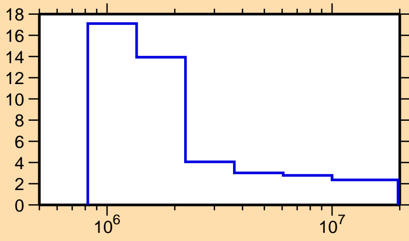
\Delta\sigma/\sigma vs. E for ^{210}\text{Bi}(n,n\text{onel.})
