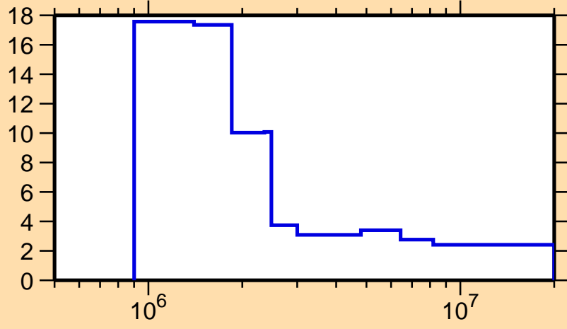
\Delta\sigma/\sigma vs. E for ^{210}\text{Bi}(n,n\text{nonel.})
