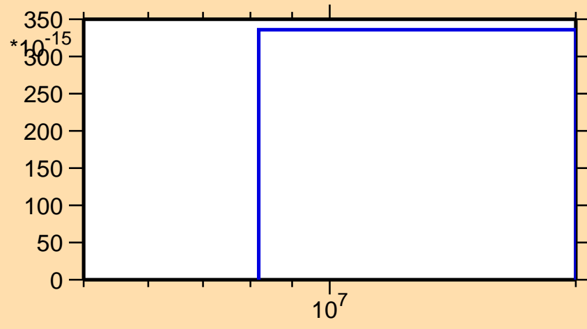
\sigma vs. E for ^{210}\text{Bi} (mt 11)
