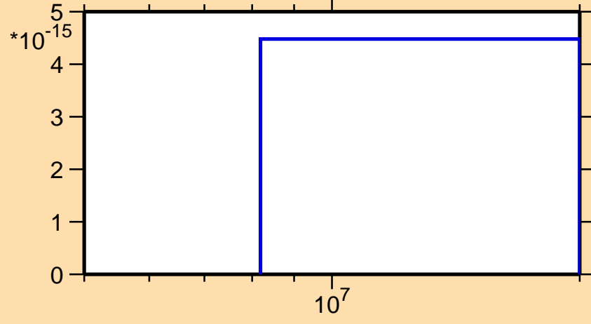
\sigma vs. E for ^{210}\text{Bi}(n,3n\alpha)
