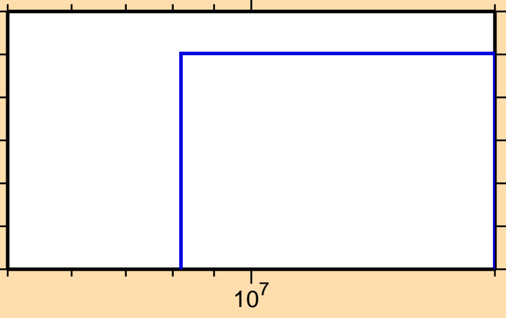
\sigma vs. E for ^{210}\text{Bi}(n,2np)
