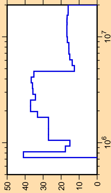
\Delta\sigma/\sigma vs. E for ^{211}\text{Bi}(n,n_3)
