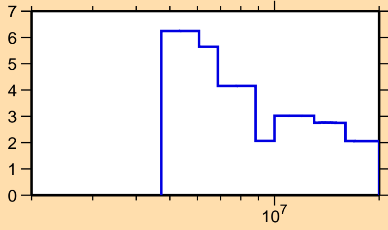
\Delta\sigma/\sigma vs. E for ^{211}\text{Bi}(n,\text{el.})
