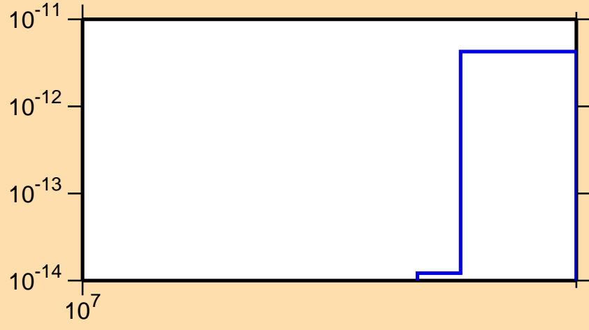
\sigma vs. E for ^{212}\text{Bi} (mt 45)
