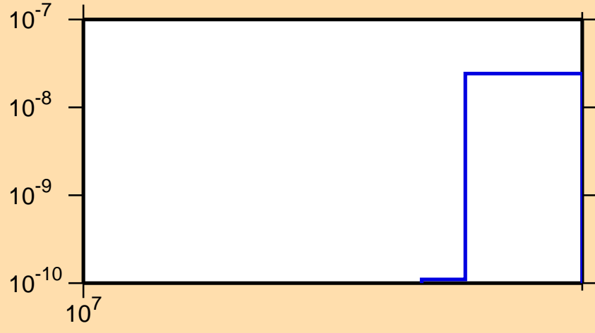
\sigma vs. E for ^{212}\text{Bi} (mt 11)
