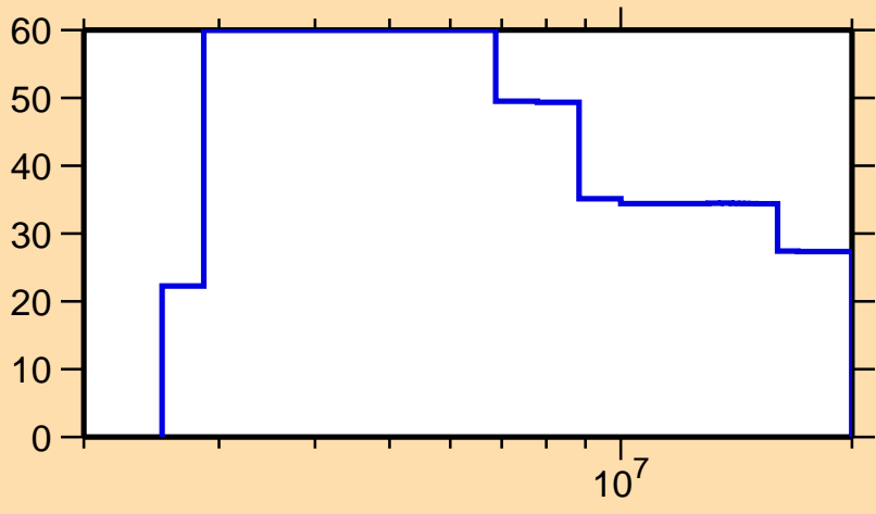
\Delta\sigma/\sigma vs. E for ^{212}\text{Bi}(n,p)
