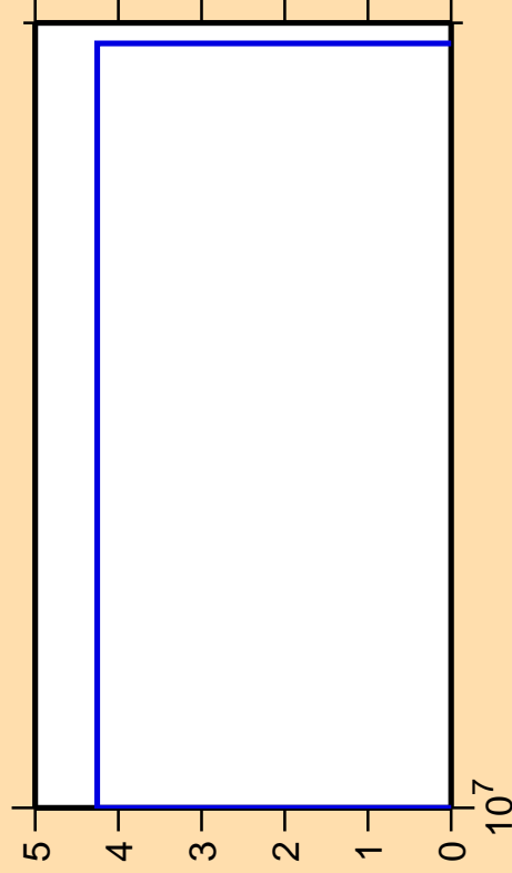
\Delta\sigma/\sigma vs. E for ^{212}\text{Bi} (mt 42)
