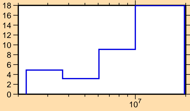
\Delta\sigma/\sigma vs. E for ^{212}\text{Bi}(n,ncont.)
