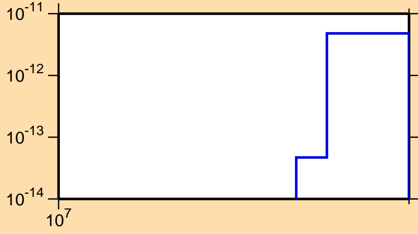
\sigma vs. E for ^{212}\text{Bi} (mt 34)
