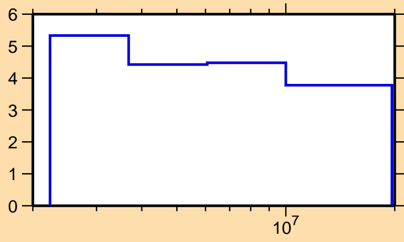
\Delta\sigma/\sigma vs. E for ^{212}\text{Bi}(n,\text{nonel.})
