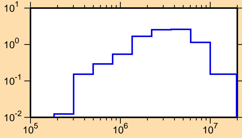
\sigma vs. E for ^{213}\text{Bi}(n,\text{inel.})
