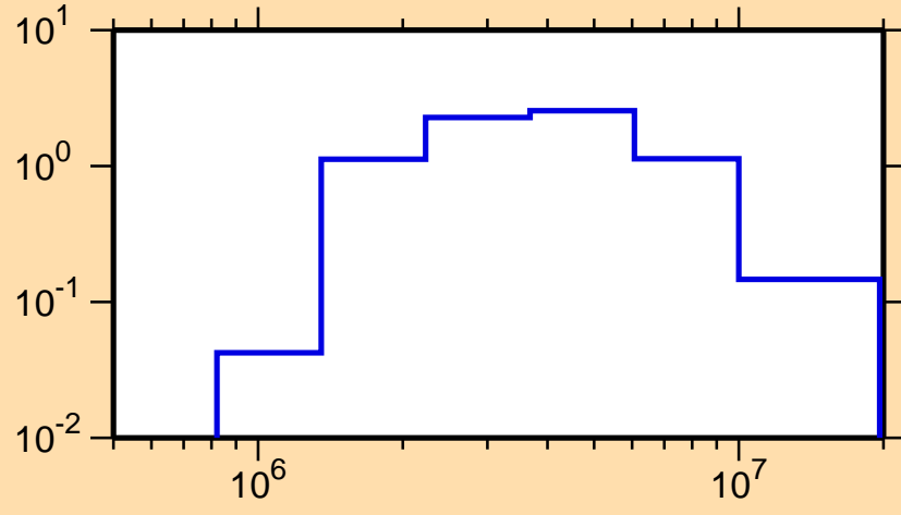
\sigma vs. E for ^{213}\text{Bi}(n,n\text{cont.})
