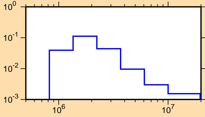
\sigma vs. E for ^{213}\text{Bi}(n,n_4)
