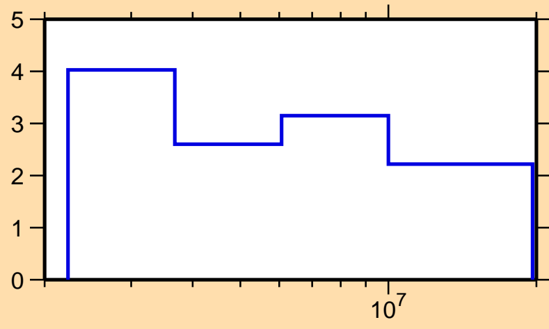
\Delta\sigma/\sigma vs. E for ^{213}\text{Bi}(n,\text{nonel.})
