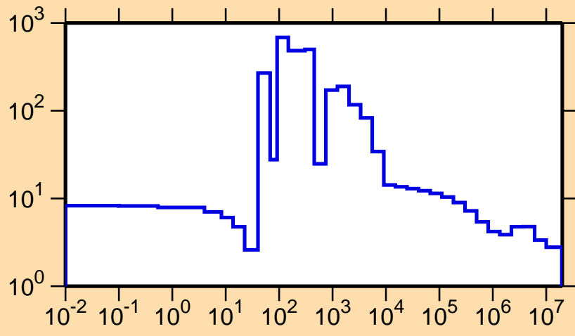
\sigma vs. E for ^{213}\text{Bi}(n,\text{el.})
