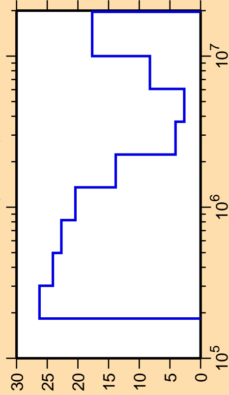
\Delta\sigma/\sigma vs. E for ^{213}\text{Bi}(n,\text{inel.})
