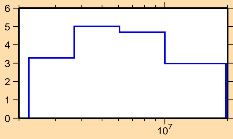
\Delta\sigma/\sigma vs. E for ^{213}\text{Bi}(n,\text{el.})
