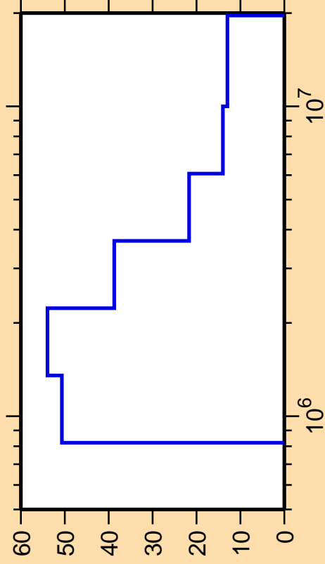
\Delta\sigma/\sigma vs. E for ^{213}\text{Bi}(n,n_4)
