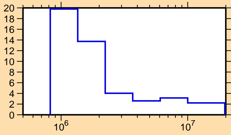
\Delta\sigma/\sigma vs. E for ^{213}\text{Bi}(n,n\text{onel.})
