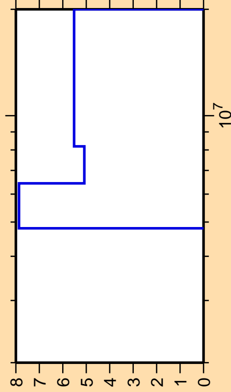
\Delta\sigma/\sigma vs. E for ^{213}\text{Bi}(n,2n)
