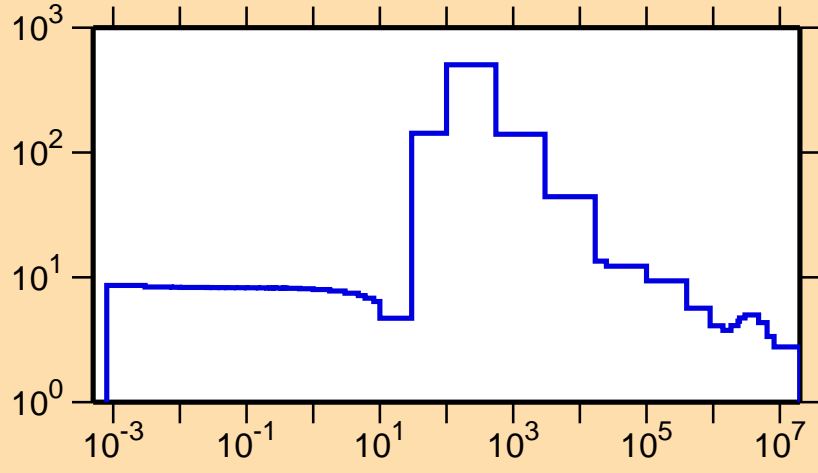
\sigma vs. E for ^{213}\text{Bi}(n,\text{el.})
