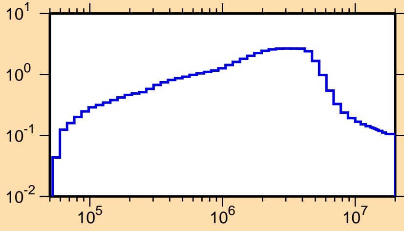
\sigma vs. E for ^{214}\text{Bi}(n,\text{inel.})
