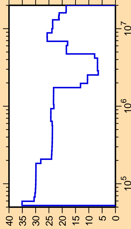
\Delta\sigma/\sigma vs. E for ^{214}\text{Bi}(n,\text{inel.})
