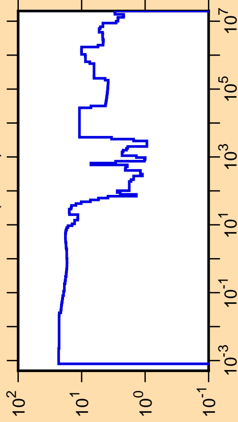
\Delta\sigma/\sigma vs. E for ^{214}\text{Bi}(n,\text{tot.})
