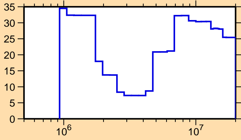
\Delta\sigma/\sigma vs. E for ^{214}\text{Bi}(n,n\text{cont.})
