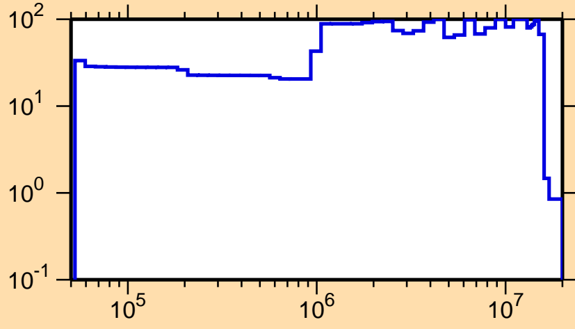
\Delta\sigma/\sigma vs. E for ^{214}\text{Bi}(n,n_1)
