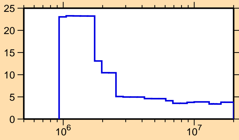
\Delta\sigma/\sigma vs. E for ^{214}\text{Bi}(n,n\text{nonel.})
