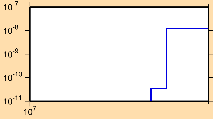
\sigma vs. E for ^{214}\text{Bi} (mt 11)
