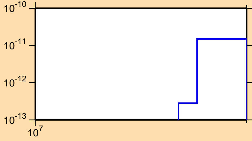
\sigma vs. E for ^{214}\text{Bi}(n,\text{He3})
