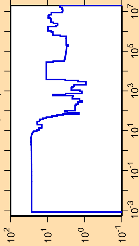
\Delta\sigma/\sigma vs. E for ^{214}\text{Bi}(n,\text{el.})
