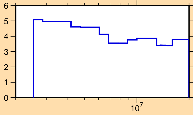
\Delta\sigma/\sigma vs. E for ^{214}\text{Bi}(n,\text{nonel.})
