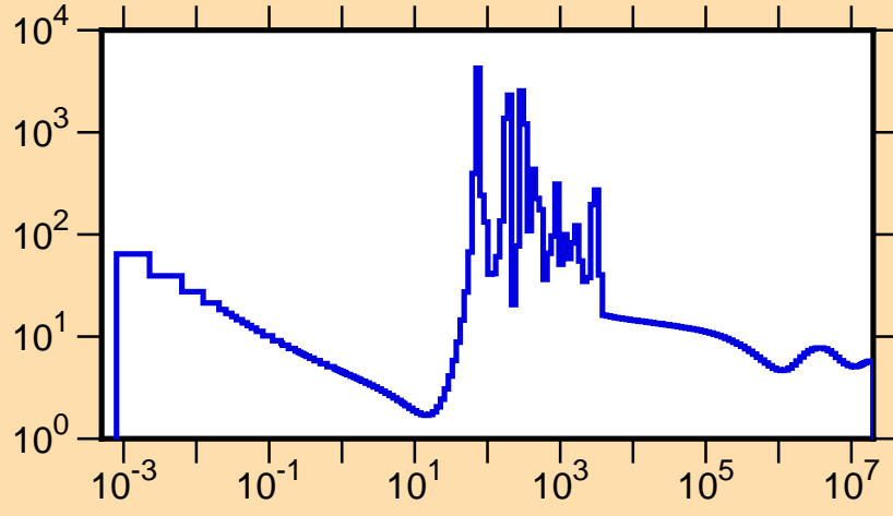
\sigma vs. E for ^{214}\text{Bi}(n,\text{tot.})
