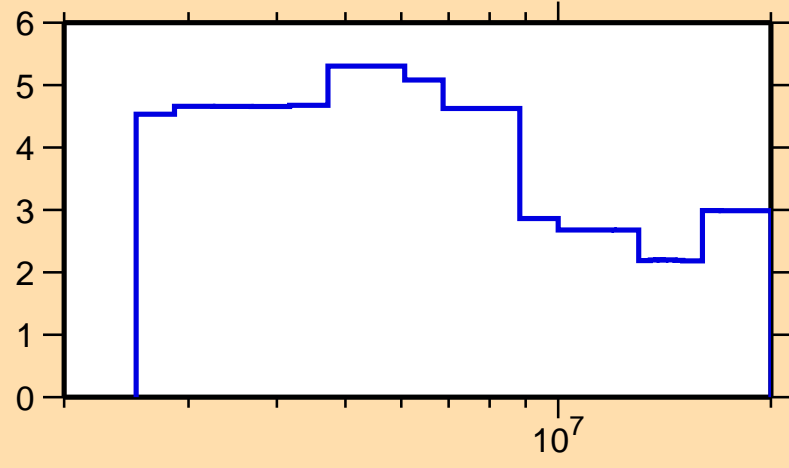
\Delta\sigma/\sigma vs. E for ^{214}\text{Bi}(n,\text{tot.})
