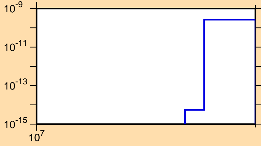
\sigma vs. E for ^{214}\text{Bi} (mt 42)
