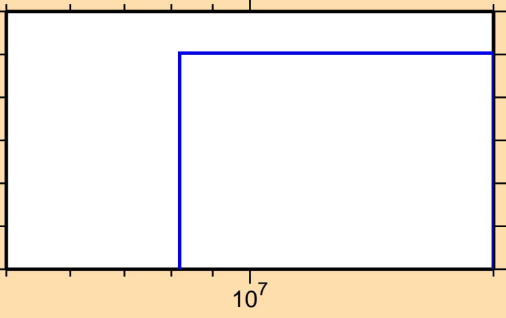
\sigma vs. E for ^{214}\text{Bi}(n,\text{nd})
