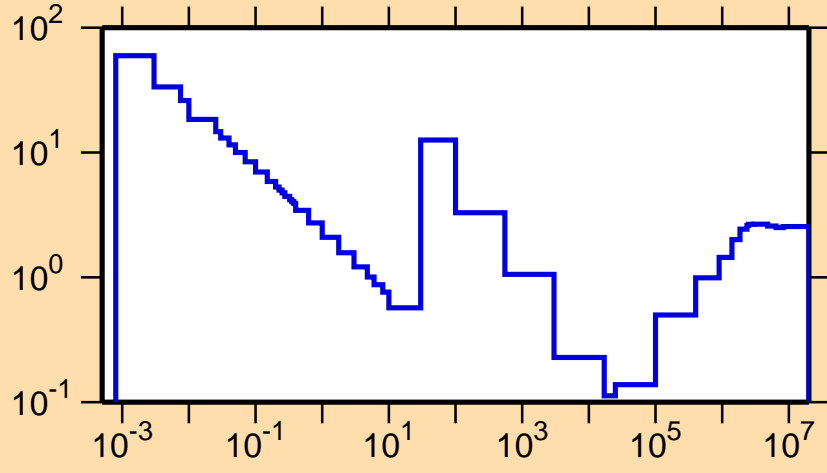
\sigma vs. E for ^{214}\text{Bi}(n,\text{nonel.})
