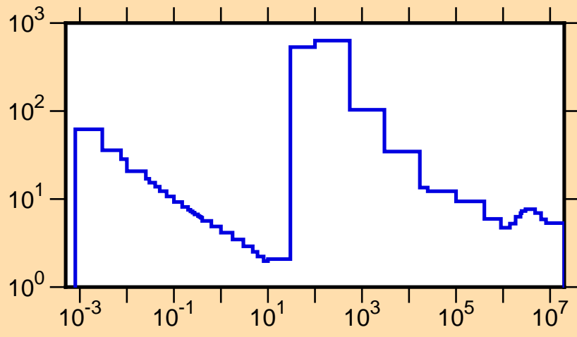
\sigma vs. E for ^{214}\text{Bi}(n,\text{tot.})
