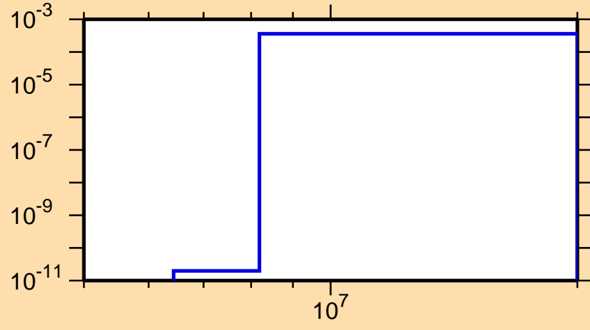
\sigma vs. E for ^{214}\text{Bi}(n,d)
