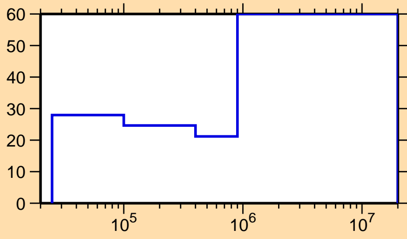
\Delta\sigma/\sigma vs. E for ^{214}\text{Bi}(n,n_1)
