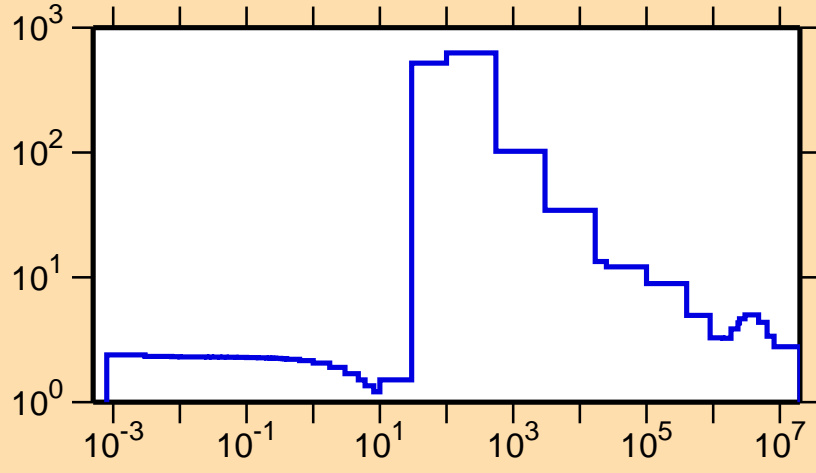
\sigma vs. E for ^{214}\text{Bi}(n,\text{el.})
