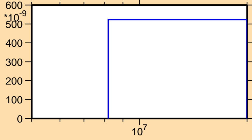
\sigma vs. E for ^{214}\text{Bi}(n,2np)
