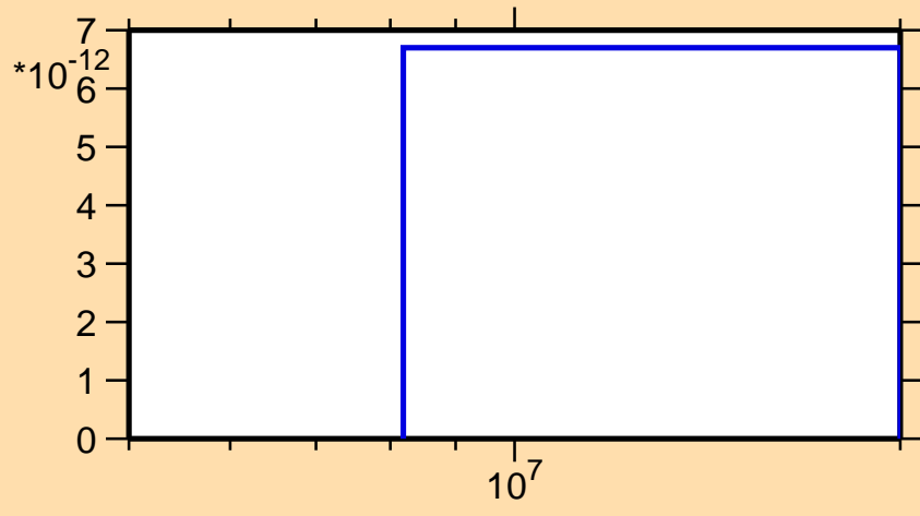
\sigma vs. E for ^{215}\text{Bi} (mt 42)
