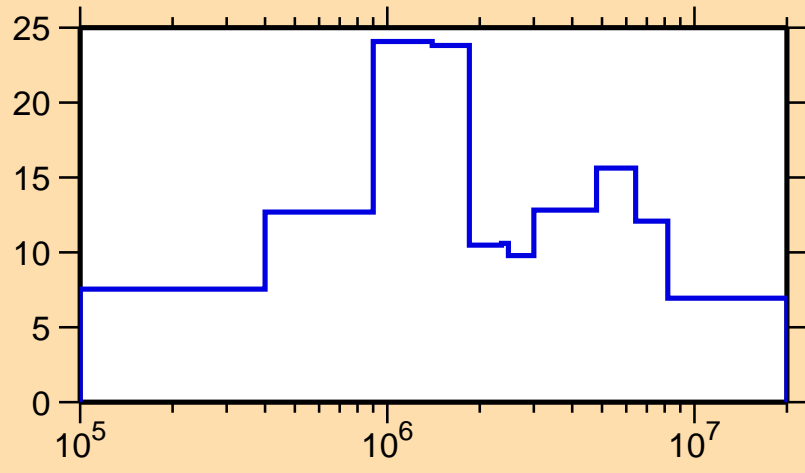
\Delta\sigma/\sigma vs. E for ^{215}\text{Bi}(n, el.)
