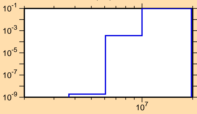
\sigma vs. E for ^{216}\text{Bi}(n,t)
