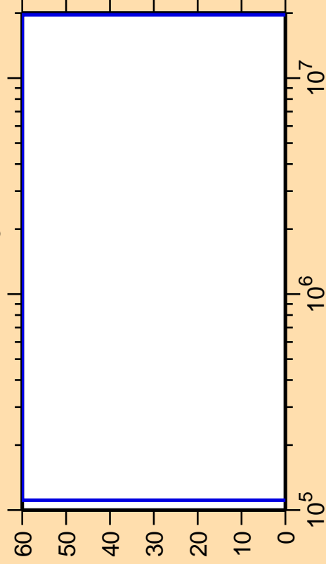
\Delta\sigma/\sigma vs. E for ^{216}\text{Bi}(n,n_3)
