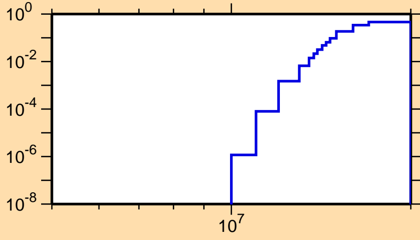
\sigma vs. E for ^{216}\text{Bi}(n,nt)
