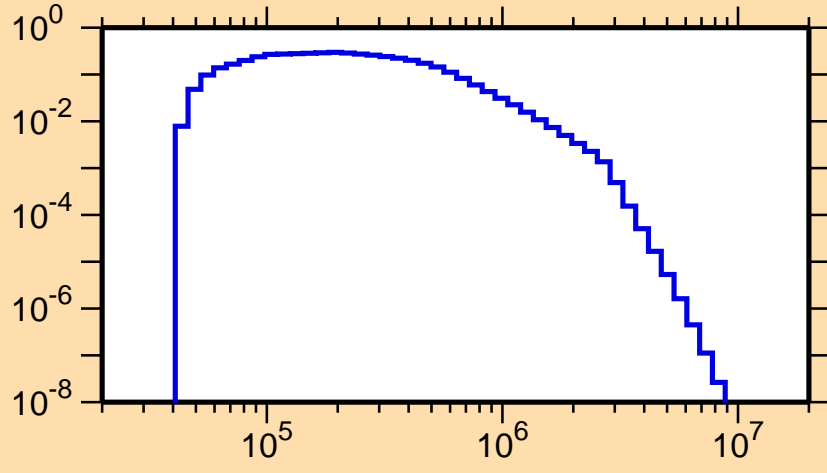
\sigma vs. E for ^{216}\text{Bi}(n,n_2)
