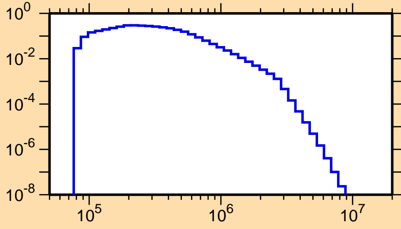
\sigma vs. E for ^{216}\text{Bi}(n,n_4)
