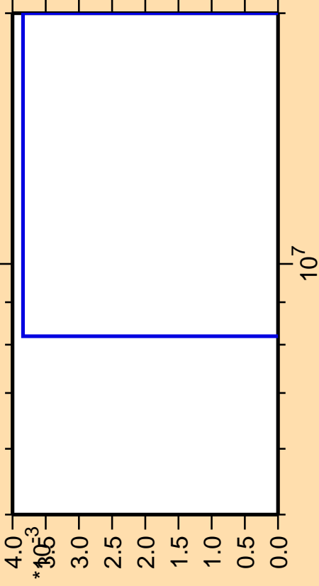
\Delta\sigma/\sigma vs. E for ^{216}\text{Bi}(n,\text{He3})
