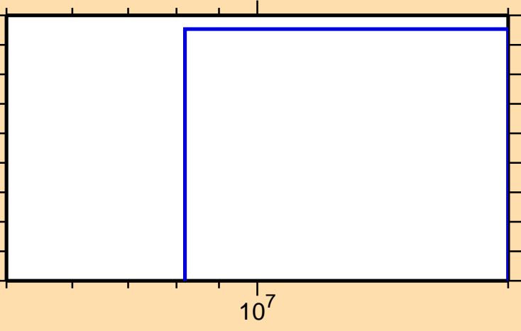
\sigma vs. E for ^{216}\text{Bi} (mt 42)
