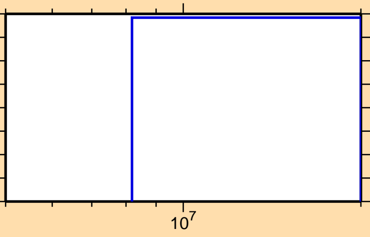
\sigma vs. E for ^{216}\text{Bi}(n,3n\alpha)
