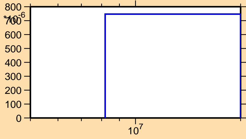
\sigma vs. E for ^{216}\text{Bi}(n,\text{nd})
