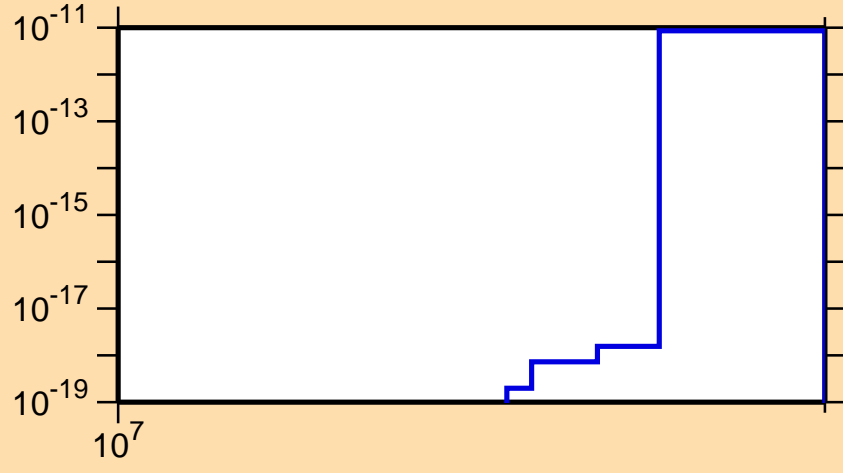
\sigma vs. E for ^{217}\text{Bi} (mt 42)
