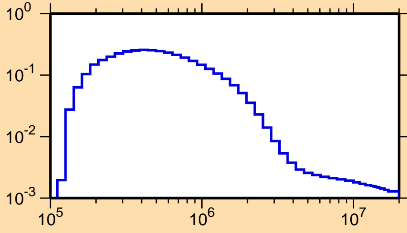
\sigma vs. E for ^{217}\text{Bi}(n,n_1)
