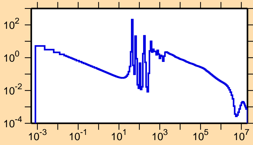
\sigma vs. E for ^{217}\text{Bi}(n,\gamma)
