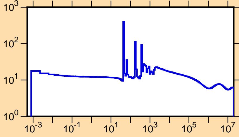
\sigma vs. E for ^{217}\text{Bi}(n,\text{tot.})
