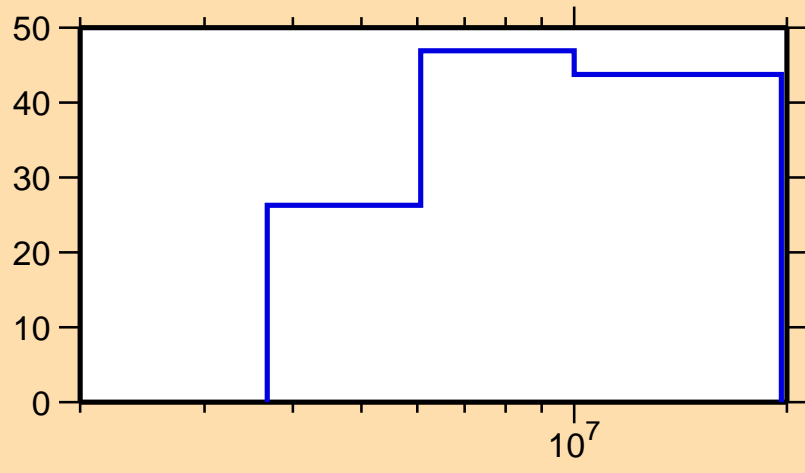
\Delta\sigma/\sigma vs. E for ^{217}\text{Bi}(n,\text{tot.})
