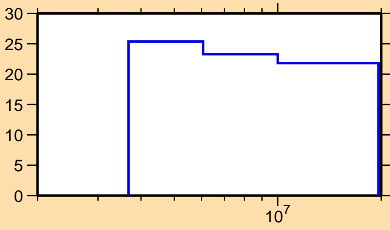
\Delta\sigma/\sigma vs. E for ^{217}\text{Bi}(n,\text{nonel.})
