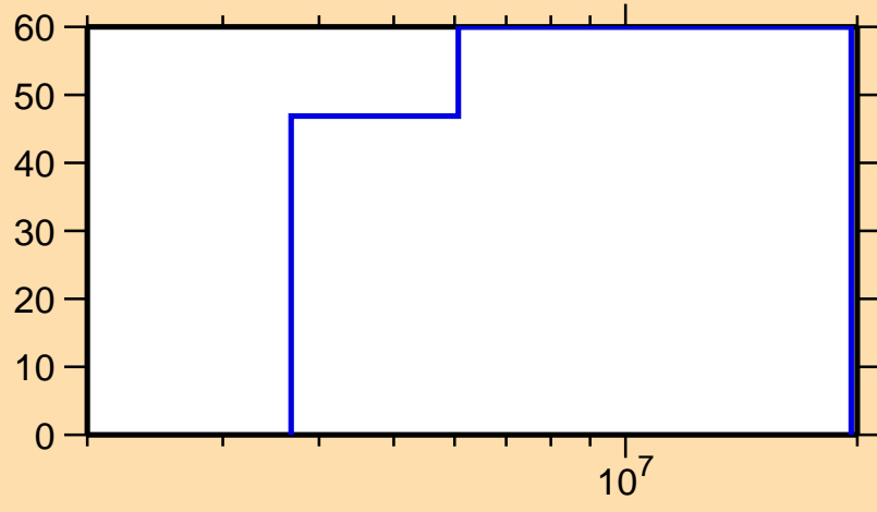
\Delta\sigma/\sigma vs. E for ^{217}\text{Bi}(n,\text{inel.})
