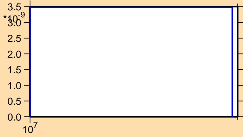
\sigma vs. E for ^{217}\text{Bi}(n,2np)
