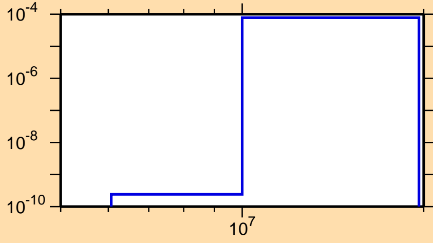
\sigma vs. E for ^{217}\text{Bi}(n,d)
