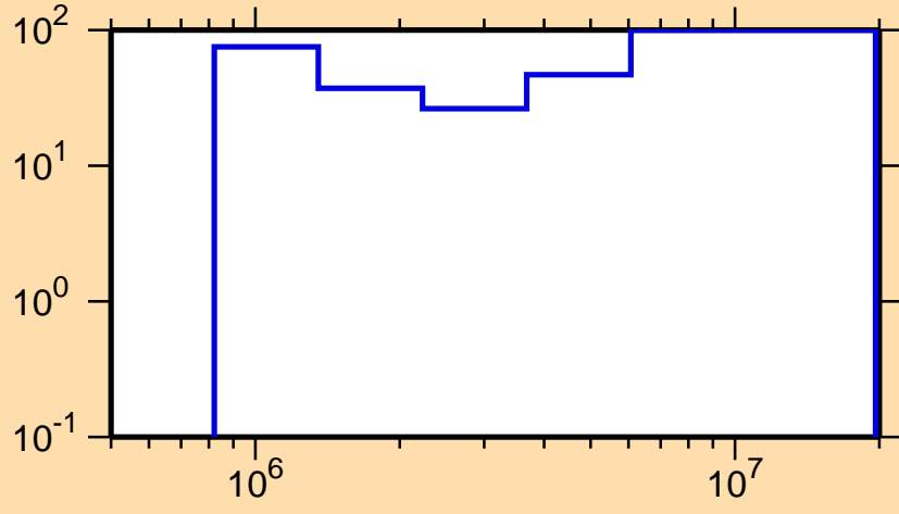
\Delta\sigma/\sigma vs. E for ^{217}\text{Bi}(n,\text{inel.})
