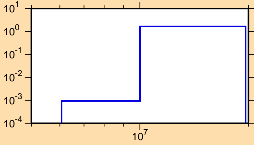
\sigma vs. E for ^{217}\text{Bi}(n,3n)
