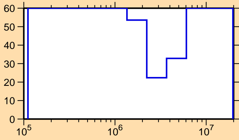
\Delta\sigma/\sigma vs. E for ^{217}\text{Bi}(n,\text{el.})
