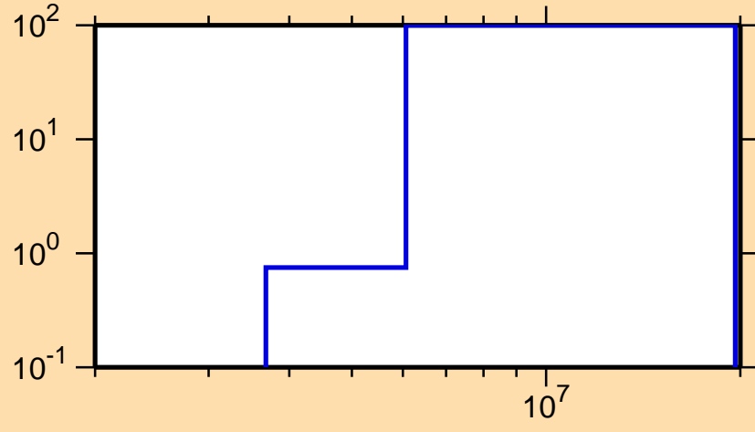
\Delta\sigma/\sigma vs. E for ^{217}\text{Bi}(n,p)
