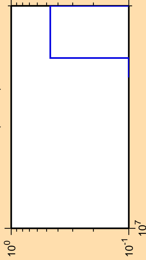
\Delta\sigma/\sigma vs. E for ^{218}\text{Bi}(n,\text{He}3)
