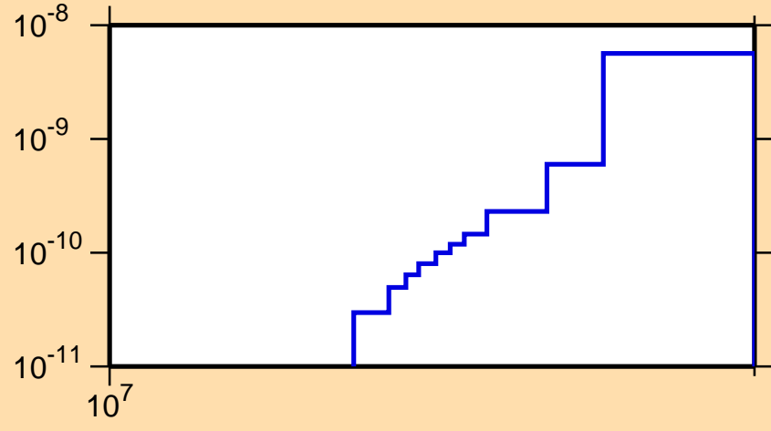
\sigma vs. E for ^{218}\text{Bi}(n,3n\alpha)
