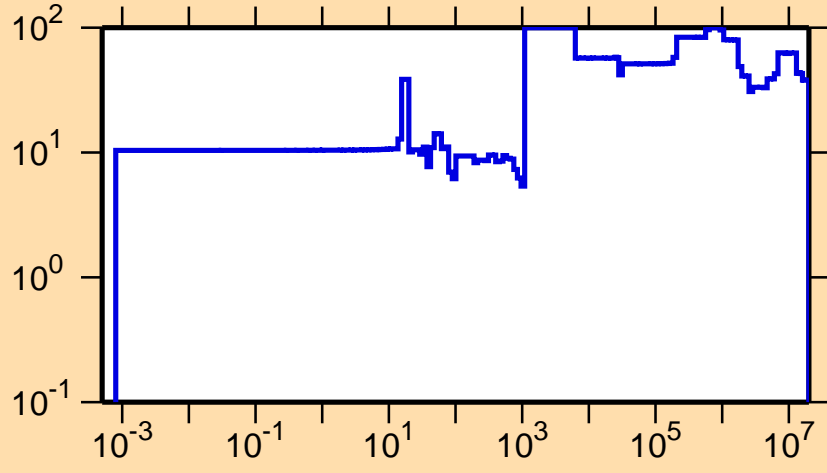
\Delta\sigma/\sigma vs. E for ^{218}\text{Bi}(n,el.)
