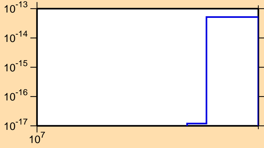
\sigma vs. E for ^{218}\text{Bi}(n,\text{He}3)
