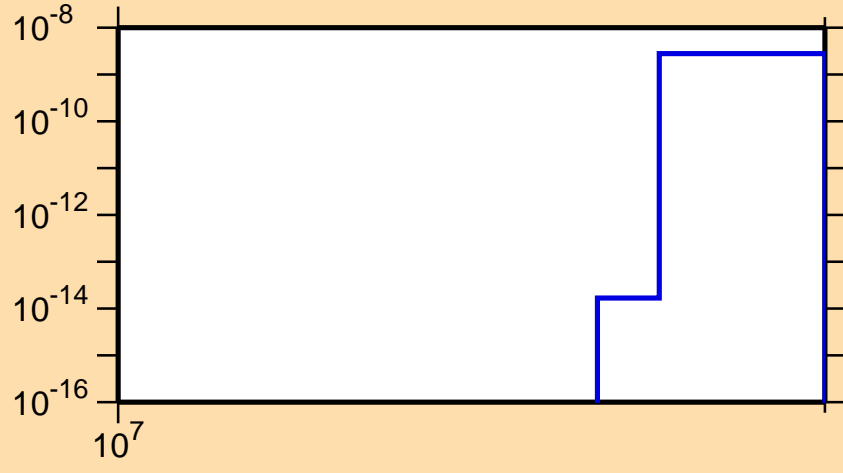
\sigma vs. E for ^{218}\text{Bi} (mt 42)
