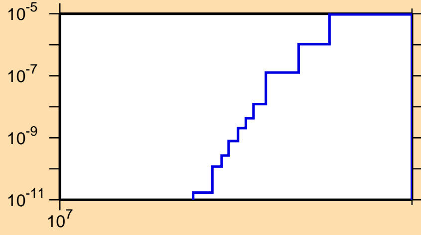
\sigma vs. E for ^{218}\text{Bi}(n,2np)
