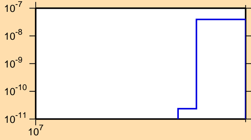
\sigma vs. E for ^{218}\text{Bi} (mt 11)
