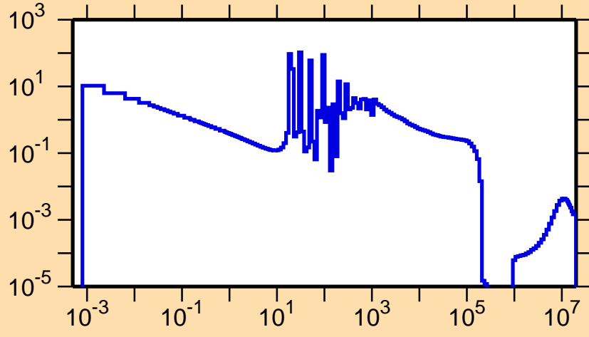
\sigma vs. E for ^{218}\text{Bi}(n,\gamma)
