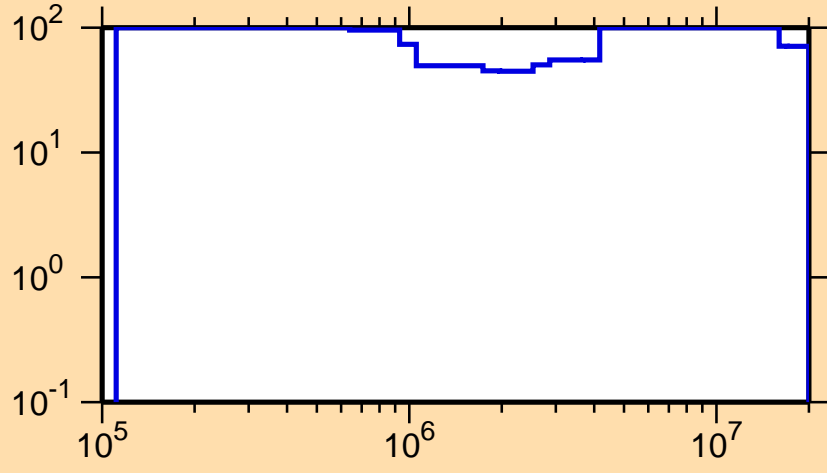
\Delta\sigma/\sigma vs. E for ^{218}\text{Bi}(n,n\text{cont.})
