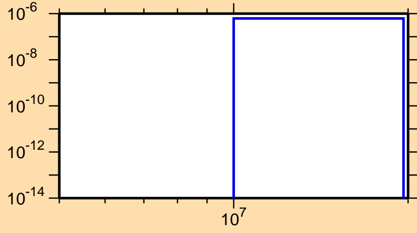
\sigma vs. E for ^{218}\text{Bi}(n,\text{nd})
