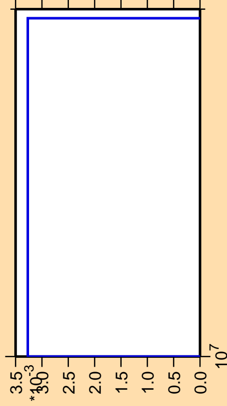
\Delta\sigma/\sigma vs. E for ^{218}\text{Bi}(n,\text{He}3)
