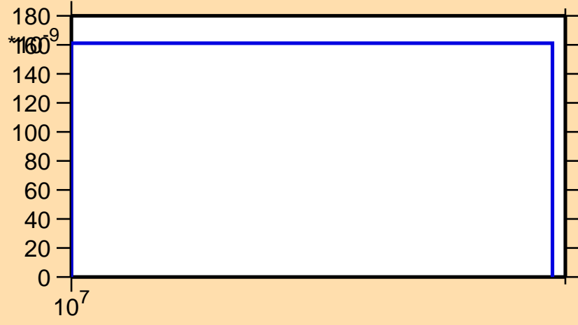
\sigma vs. E for ^{218}\text{Bi}(n,2np)
