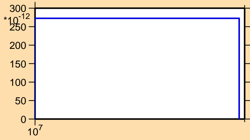
\sigma vs. E for ^{218}\text{Bi} (mt 11)
