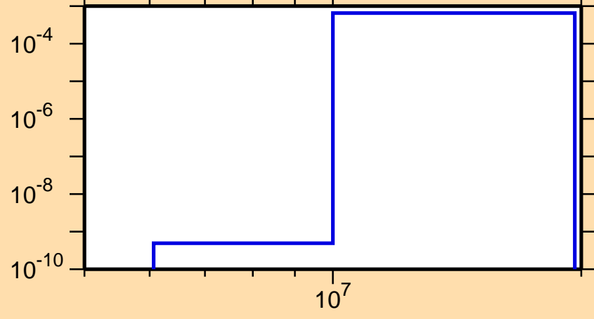
\sigma vs. E for ^{218}\text{Bi}(n,d)
