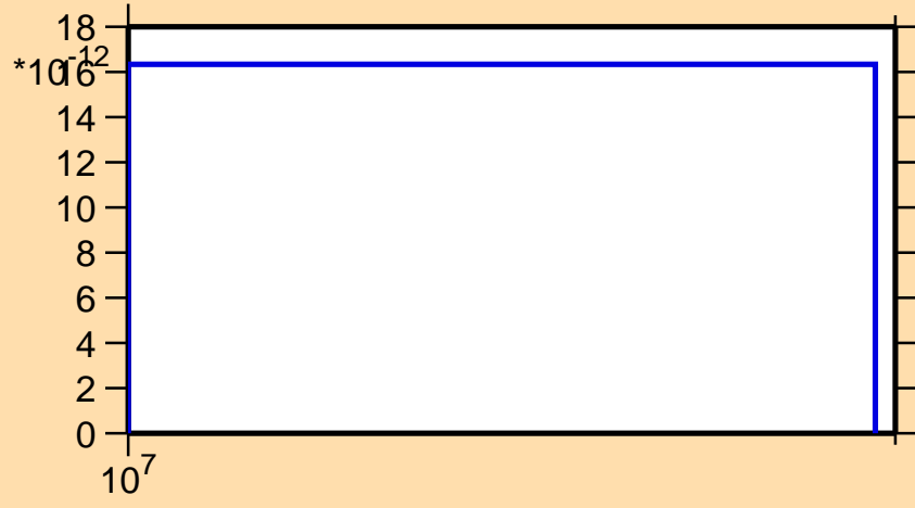
\sigma vs. E for ^{218}\text{Bi} (mt 42)
