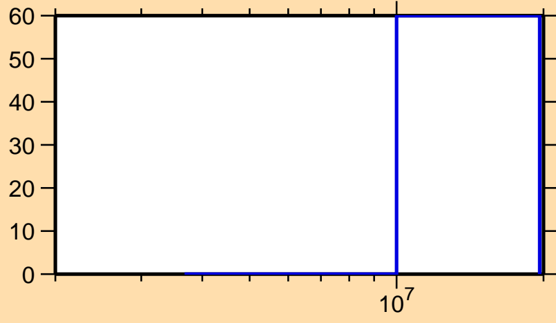
\Delta\sigma/\sigma vs. E for ^{218}\text{Bi}(n,f)
