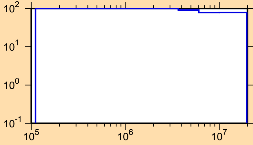
\Delta\sigma/\sigma vs. E for ^{218}\text{Bi}(n,n_1)
