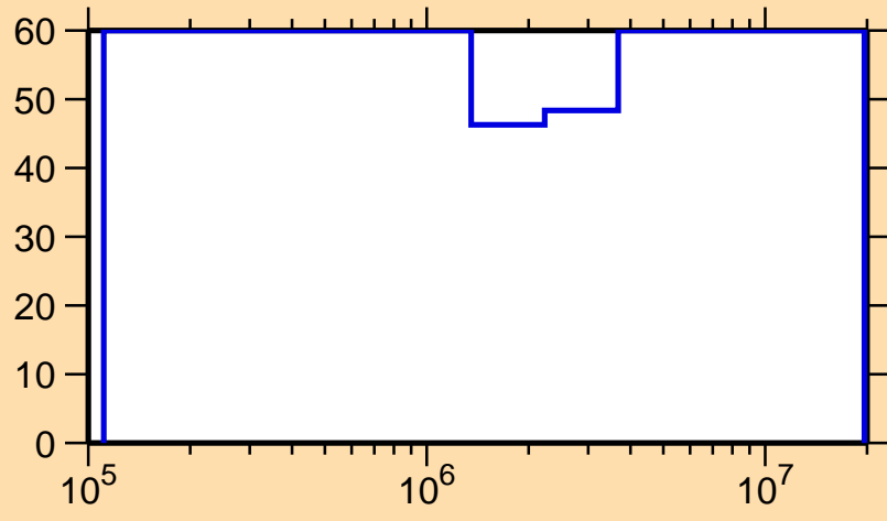
\Delta\sigma/\sigma vs. E for ^{218}\text{Bi}(n,n\text{cont.})
