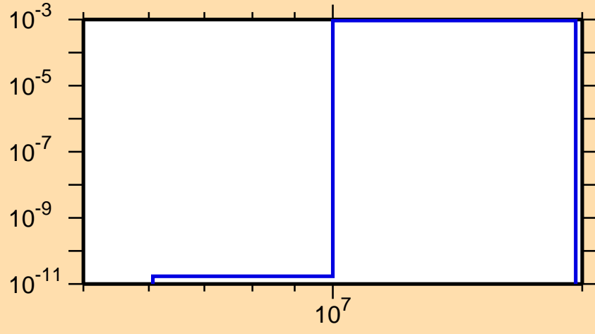
\sigma vs. E for ^{218}\text{Bi}(n,np)
