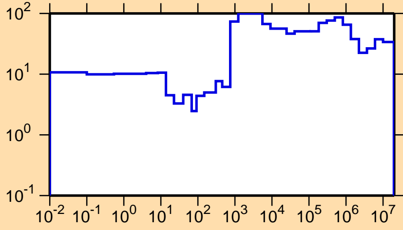
\Delta\sigma/\sigma vs. E for ^{218}\text{Bi}(n,\text{tot.})
