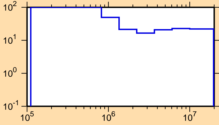
\Delta\sigma/\sigma vs. E for ^{218}\text{Bi}(n,\text{nonel.})
