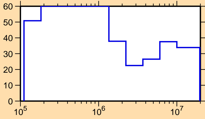
\Delta\sigma/\sigma vs. E for ^{218}\text{Bi}(n,\text{tot.})
