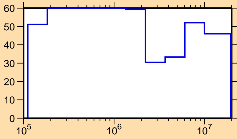
\Delta\sigma/\sigma vs. E for ^{218}\text{Bi}(n,\text{el.})
