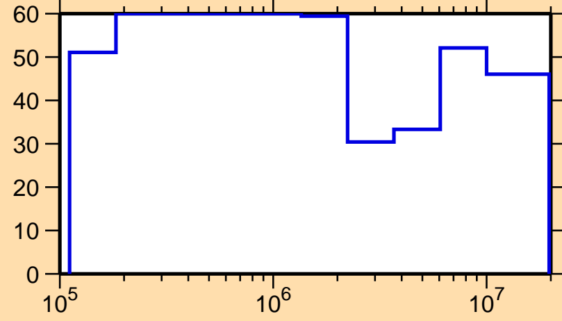
\Delta\sigma/\sigma vs. E for ^{218}\text{Bi}(n,\text{el.})
