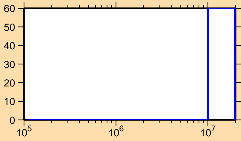
\Delta\sigma/\sigma vs. E for ^{218}\text{Bi}(n,f)
