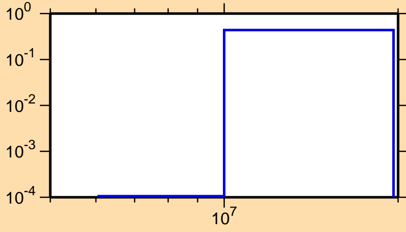
\sigma vs. E for ^{218}\text{Bi}(n,3n)
