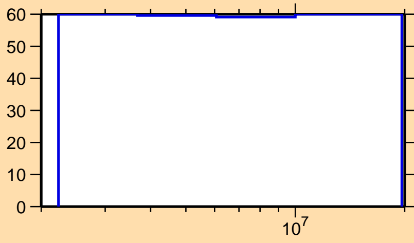
\Delta\sigma/\sigma vs. E for ^{218}\text{Bi}(n,2n)
