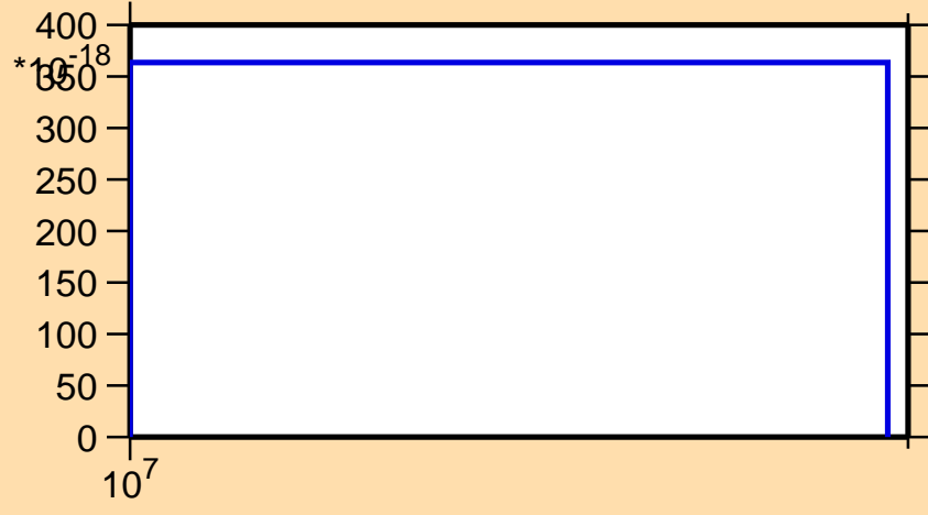
\sigma vs. E for ^{218}\text{Bi}(n,\text{He}3)
