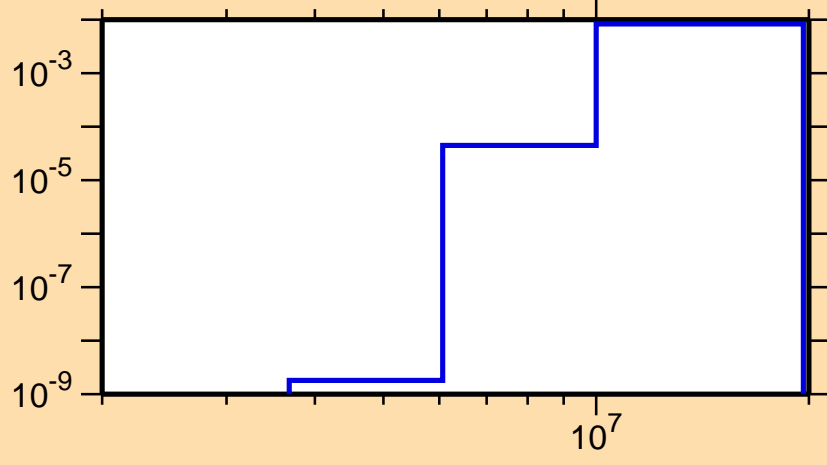
\sigma vs. E for ^{218}\text{Bi}(n,p)
