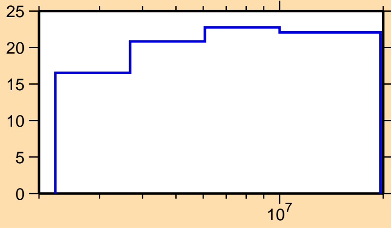
\Delta\sigma/\sigma vs. E for ^{218}\text{Bi}(n,\text{nonel.})
