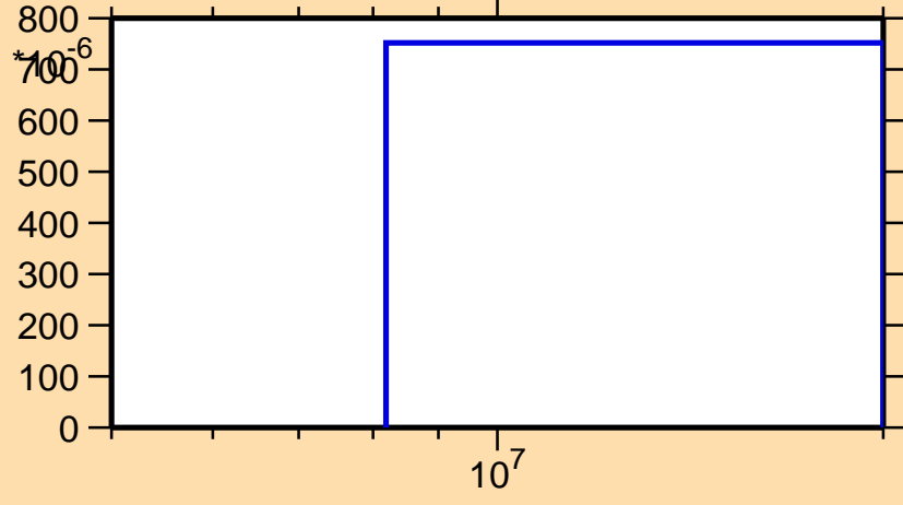
\sigma vs. E for ^{218}\text{Bi}(n,np)
