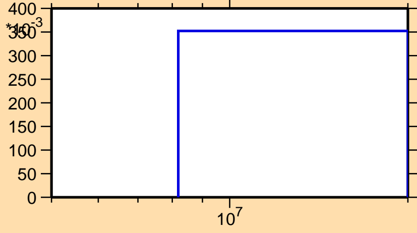
\sigma vs. E for ^{218}\text{Bi}(n,3n)
