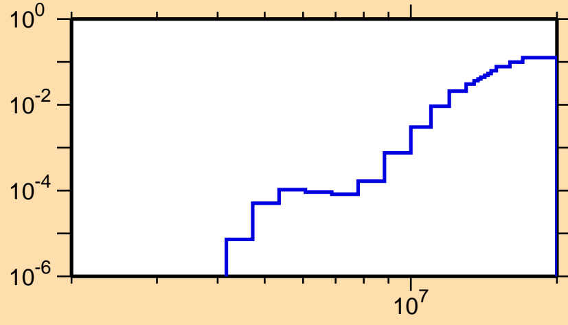
\sigma vs. E for ^{219}\text{Bi}(n,n\alpha)
