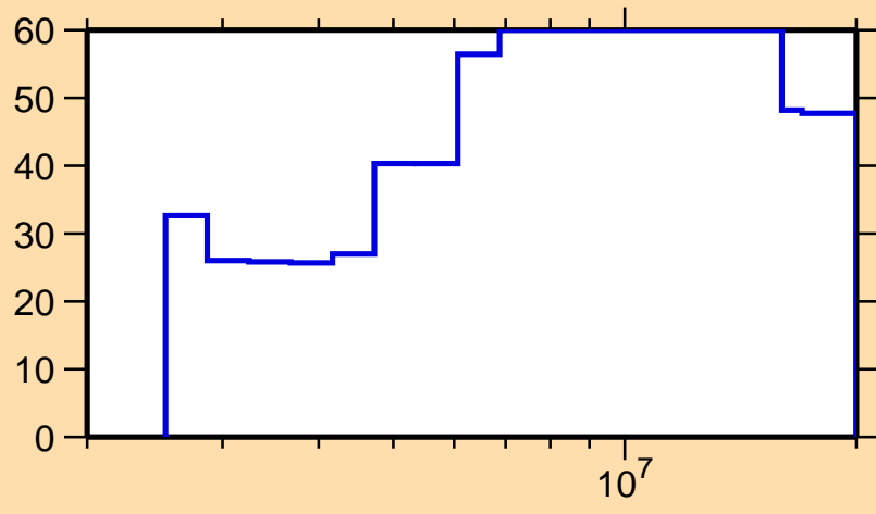
\Delta\sigma/\sigma vs. E for ^{219}\text{Bi}(n,\text{el.})
