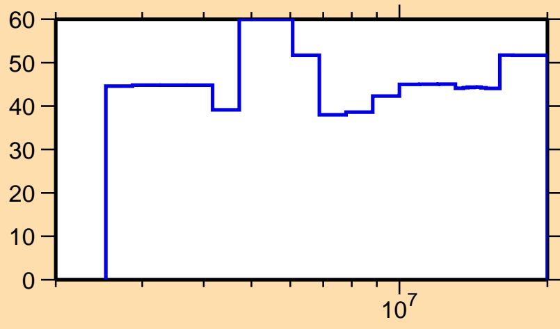
\Delta\sigma/\sigma vs. E for ^{219}\text{Bi}(n,\text{inel.})
