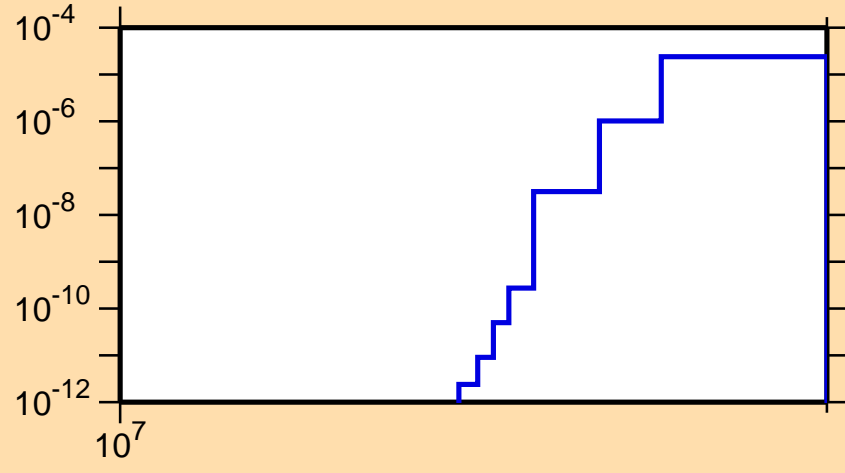
\sigma vs. E for ^{219}\text{Bi}(n,2np)
