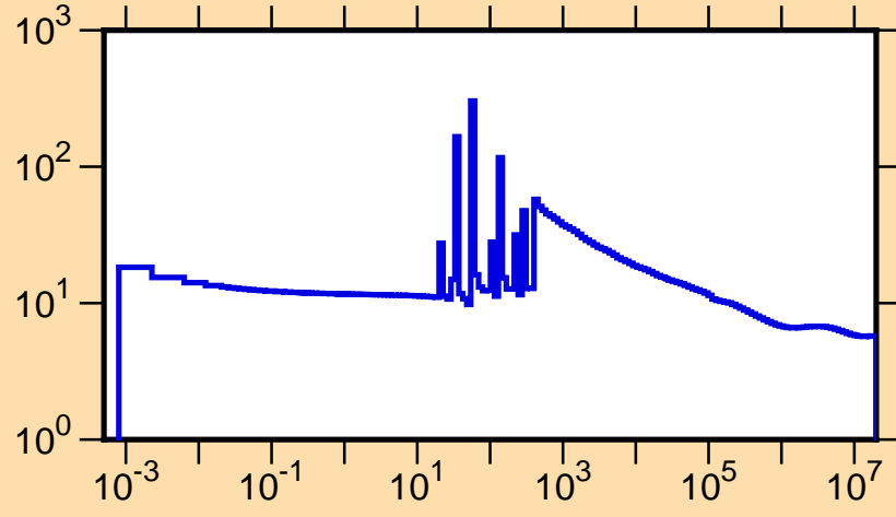
\sigma vs. E for ^{219}\text{Bi}(n,\text{tot.})
