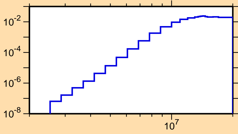
\sigma vs. E for ^{219}\text{Bi}(n,\alpha)
