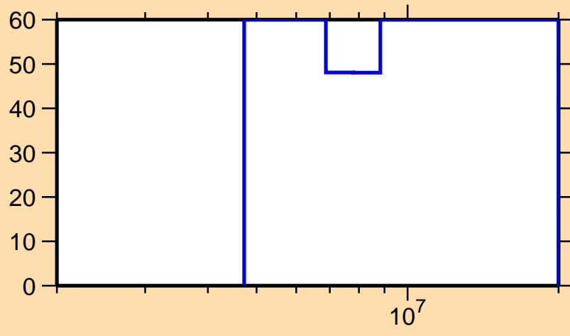
\Delta\sigma/\sigma vs. E for ^{219}\text{Bi}(n,2n)
