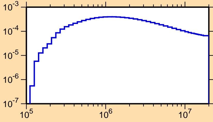
\sigma vs. E for ^{219}\text{Bi}(n,n_1)
