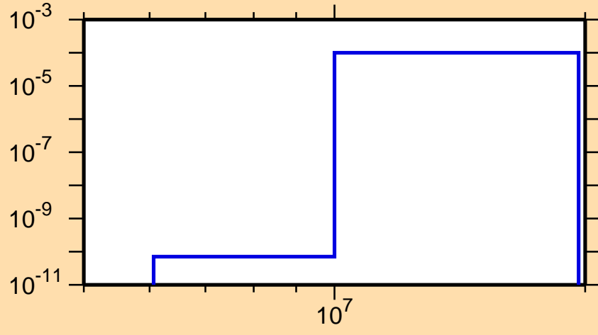
\sigma vs. E for ^{219}\text{Bi}(n,t)
