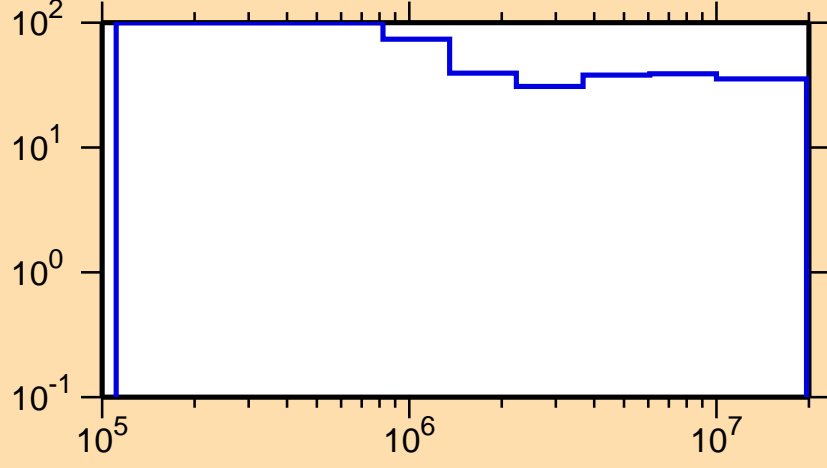
\Delta\sigma/\sigma vs. E for ^{219}\text{Bi}(n,n\text{nonel.})
