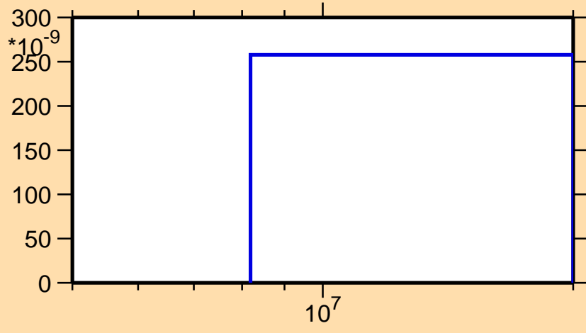
\sigma vs. E for ^{219}\text{Bi}(n,\text{nd})
