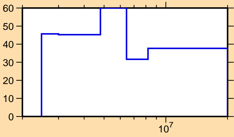
\Delta\sigma/\sigma vs. E for ^{219}\text{Bi}(n,n\text{cont.})
