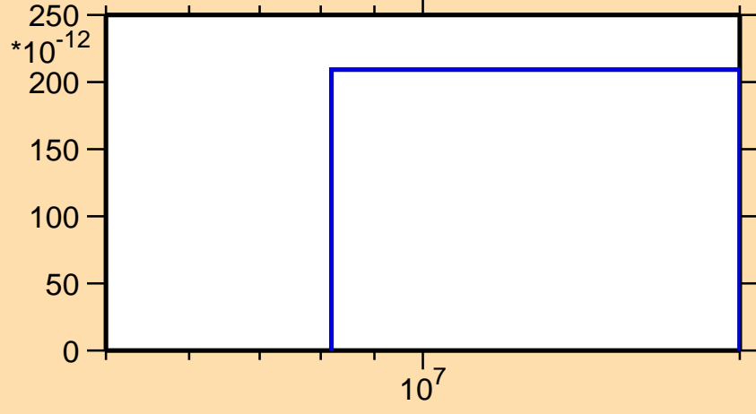
\sigma vs. E for ^{219}\text{Bi} (mt 11)
