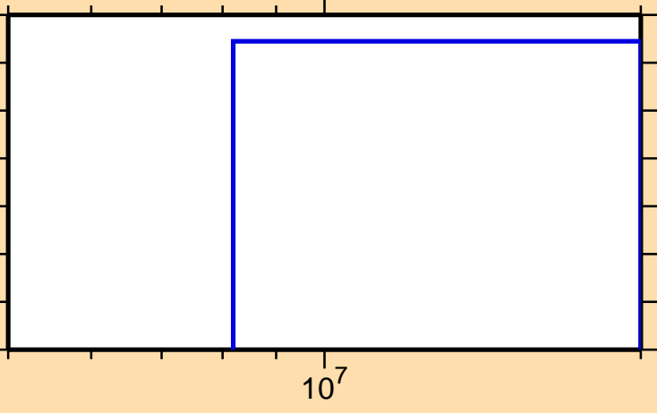
\sigma vs. E for ^{219}\text{Bi}(n,nt)
