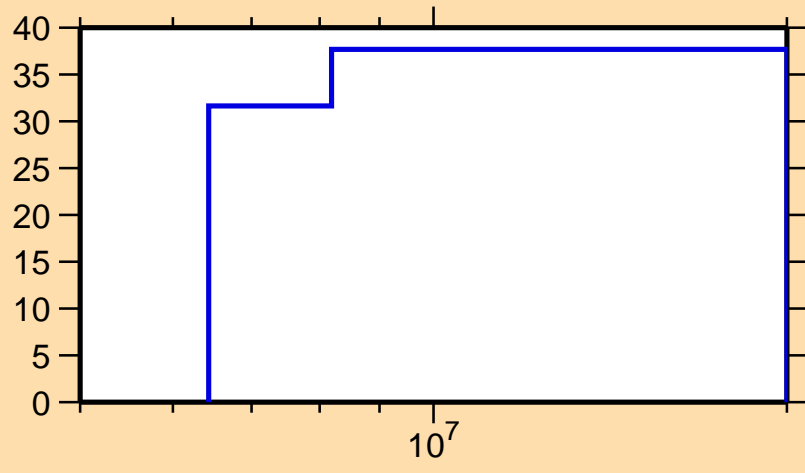
\Delta\sigma/\sigma vs. E for ^{219}\text{Bi}(n,ncont.)
