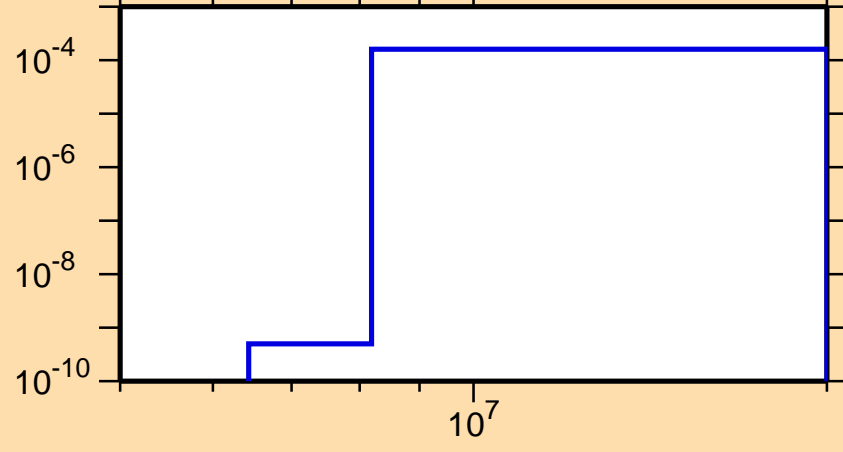
\sigma vs. E for ^{219}\text{Bi}(n,p)
