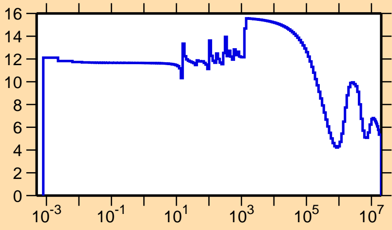
\sigma vs. E for ^{220}\text{Bi}(n,\text{el.})
