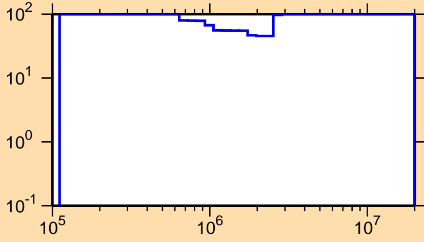
\Delta\sigma/\sigma vs. E for ^{220}\text{Bi}(n,n\text{cont.})
