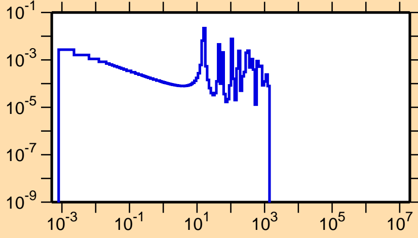
\sigma vs. E for ^{220}\text{Bi}(n,f)
