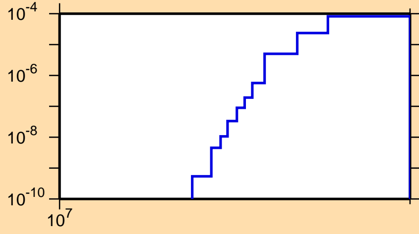
\sigma vs. E for ^{220}\text{Bi}(n,2np)
