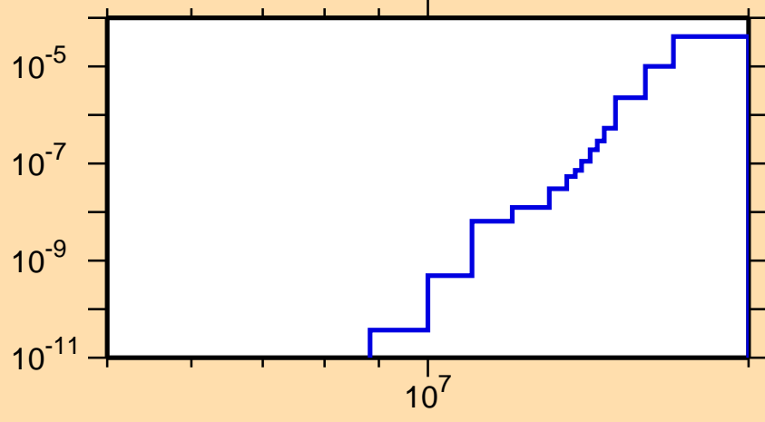
\sigma vs. E for ^{220}\text{Bi}(n,2n\alpha)
