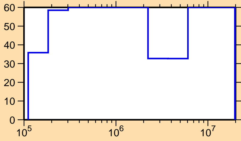
\Delta\sigma/\sigma vs. E for ^{220}\text{Bi}(n,\text{tot.})
