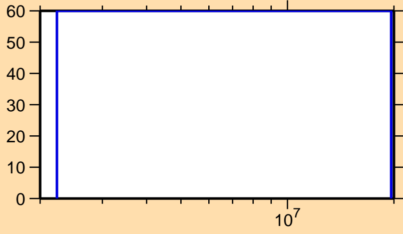
\Delta\sigma/\sigma vs. E for ^{220}\text{Bi}(n,n_1)
