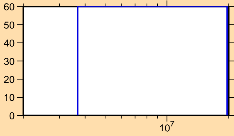
\Delta\sigma/\sigma vs. E for ^{220}\text{Bi}(n,ncont.)
