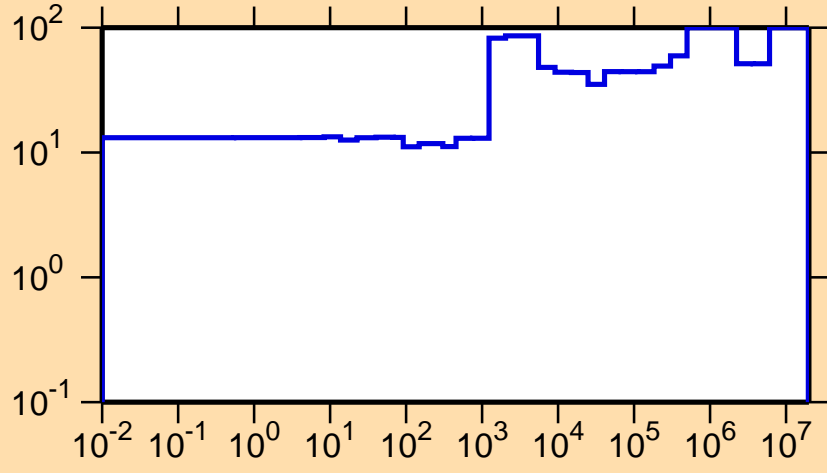
\Delta\sigma/\sigma vs. E for ^{220}\text{Bi}(n,\text{el.})
