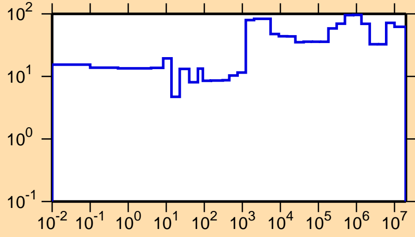
\Delta\sigma/\sigma vs. E for ^{220}\text{Bi}(n,\text{tot.})
