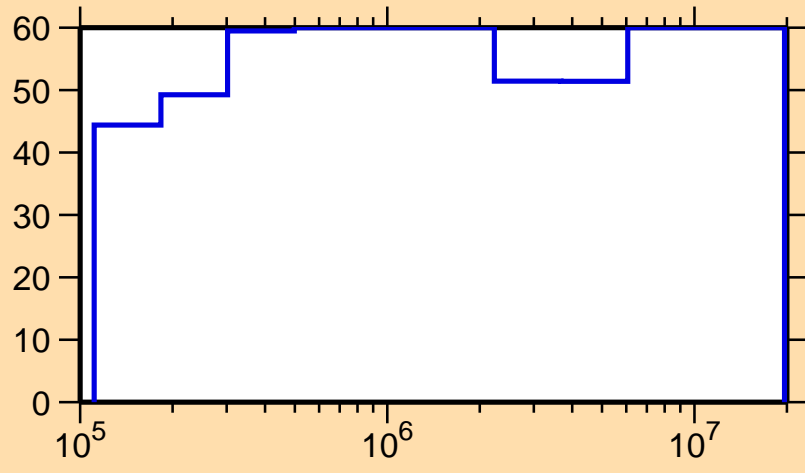
\Delta\sigma/\sigma vs. E for ^{220}\text{Bi}(n,\text{el.})
