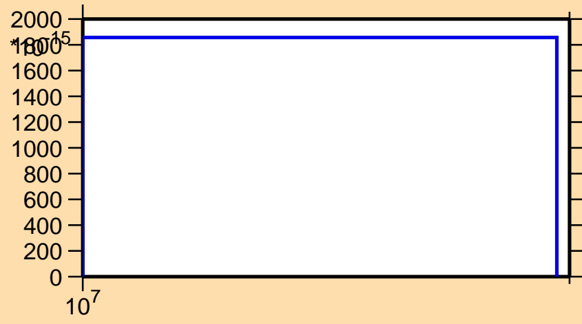
\sigma vs. E for ^{220}\text{Bi} (mt 42)
