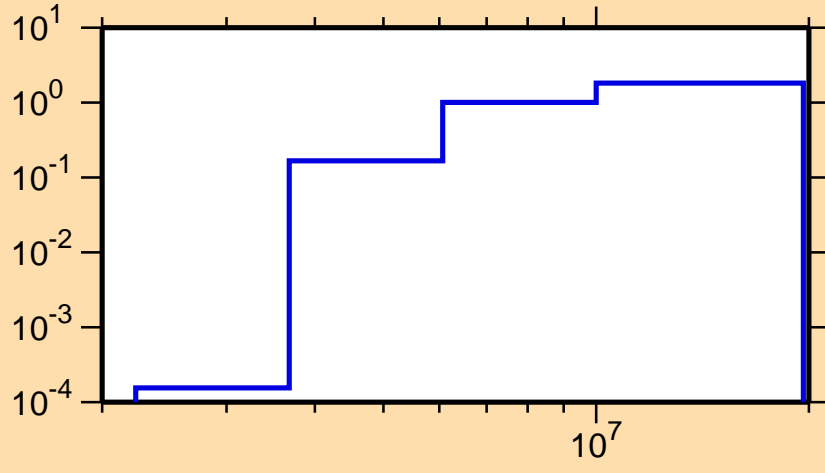
\sigma vs. E for ^{220}\text{Bi}(n,2n)
