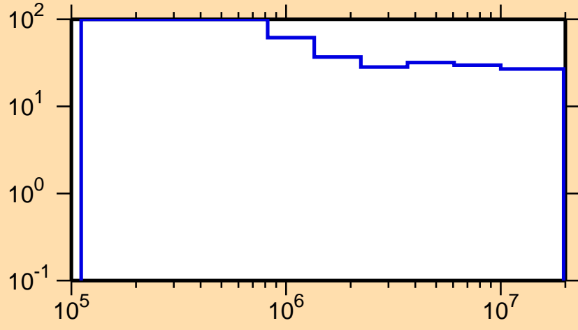
\Delta\sigma/\sigma vs. E for ^{220}\text{Bi}(n,\text{nonel.})
