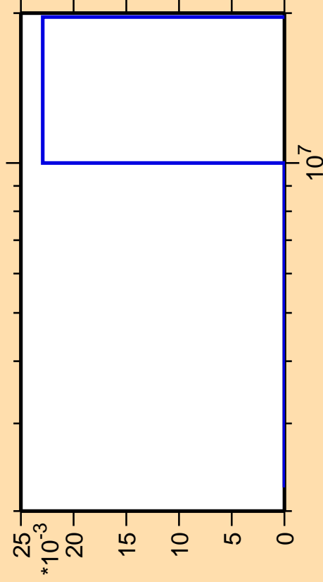
\Delta\sigma/\sigma vs. E for ^{220}\text{Bi}(n,f)
