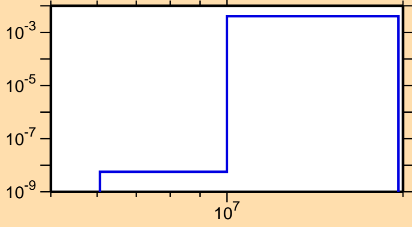
\sigma vs. E for ^{220}\text{Bi}(n,3n)
