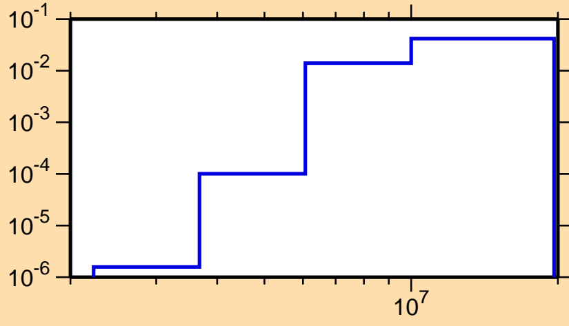
\sigma vs. E for ^{220}\text{Bi}(n,\alpha)
