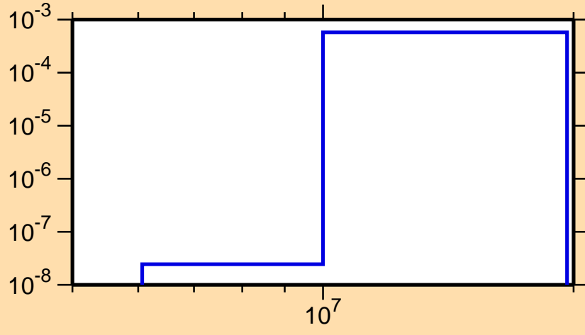
\sigma vs. E for ^{220}\text{Bi}(n,t)
