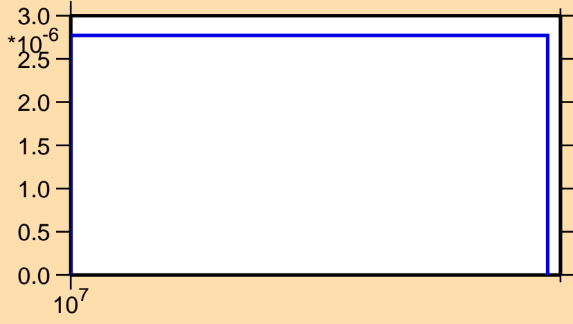
\sigma vs. E for ^{220}\text{Bi}(n,2np)
