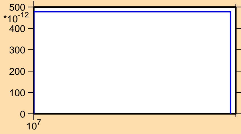
\sigma vs. E for ^{220}\text{Bi}(n,3n\alpha)
