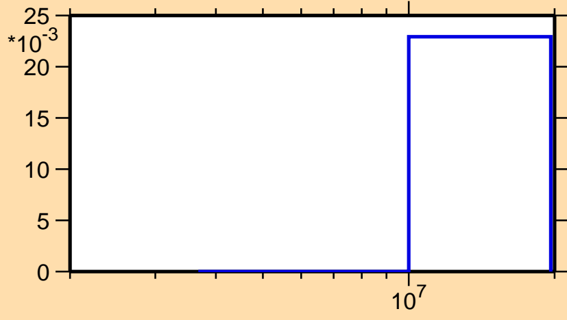
\Delta\sigma/\sigma vs. E for ^{220}\text{Bi}(n,f)
