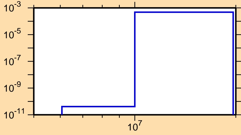
\sigma vs. E for ^{220}\text{Bi}(n,d)
