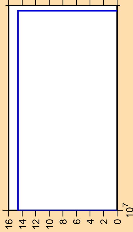
\Delta\sigma/\sigma vs. E for ^{220}\text{Bi} (mt 42)
