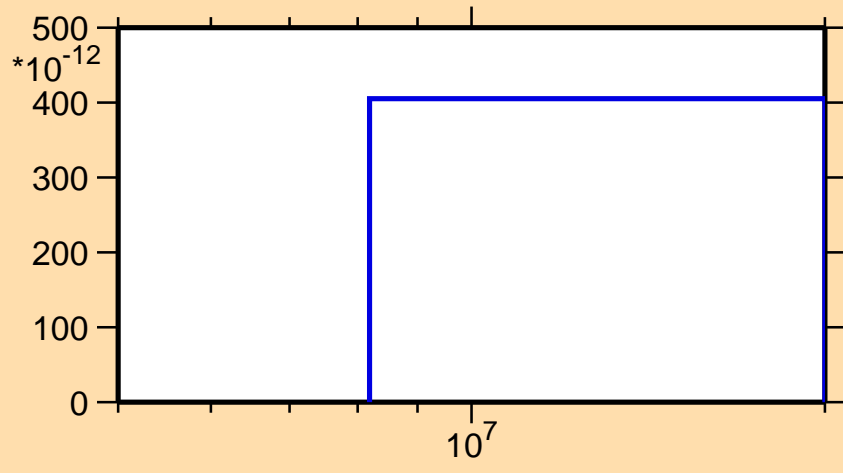
\sigma vs. E for ^{220}\text{Bi}(n,3n\alpha)
