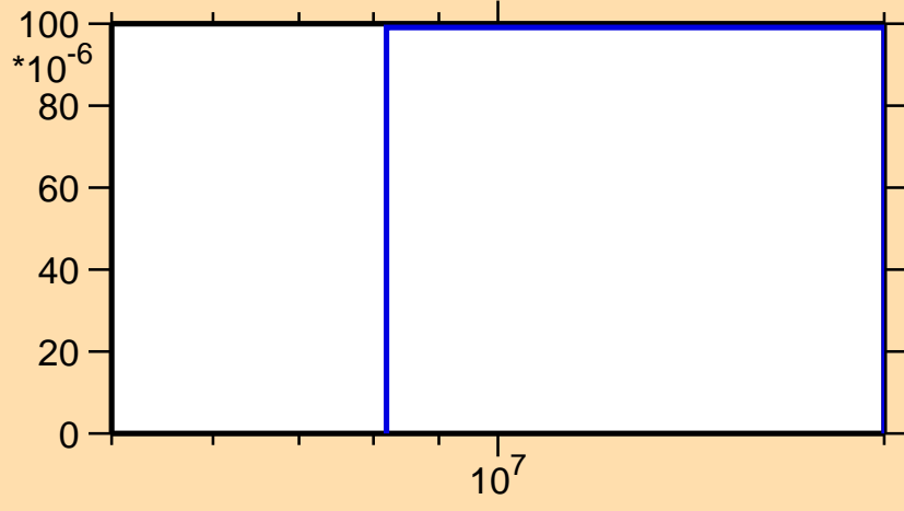
\sigma vs. E for ^{220}\text{Bi}(n,nt)
