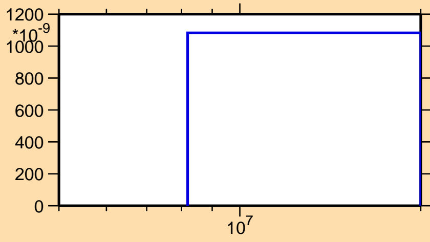
\sigma vs. E for ^{220}\text{Bi}(n,2n\alpha)
