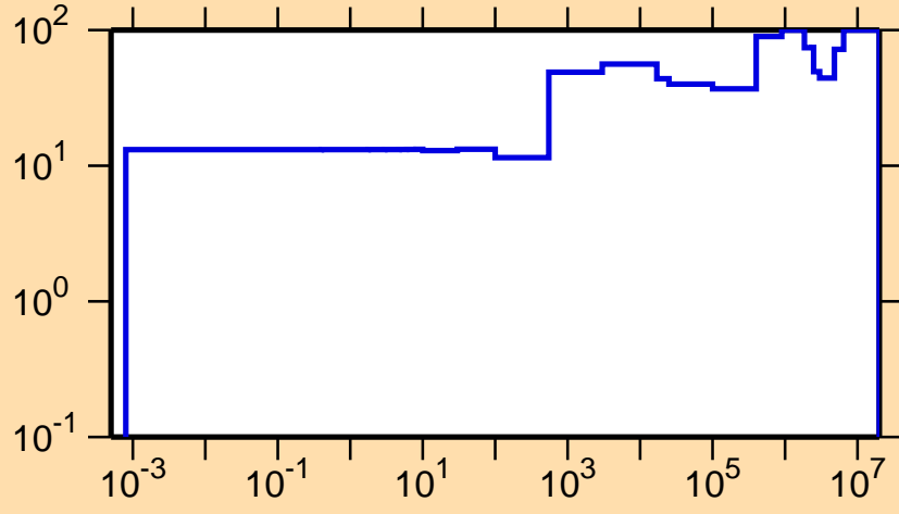
\Delta\sigma/\sigma vs. E for ^{220}\text{Bi}(n,el.)
