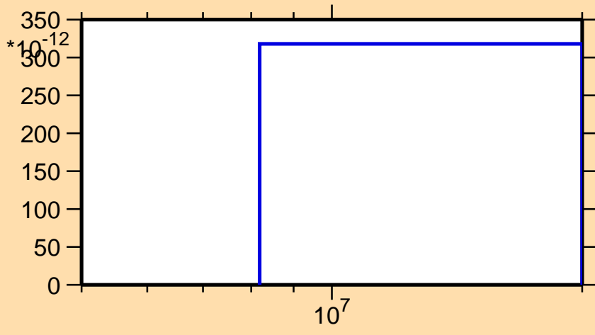
\sigma vs. E for ^{220}\text{Bi} (mt 11)
