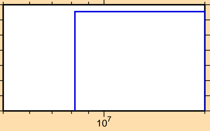
\sigma vs. E for ^{220}\text{Bi}(n,3n)
