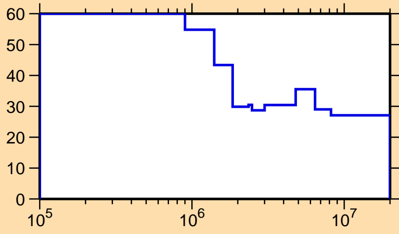
\Delta\sigma/\sigma vs. E for ^{220}\text{Bi}(n,\text{nonel.})
