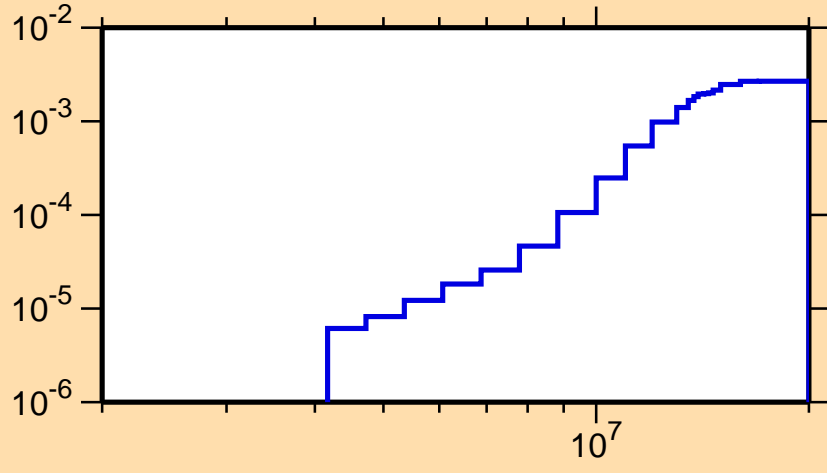
\sigma vs. E for ^{221}\text{Bi}(n,\alpha)
