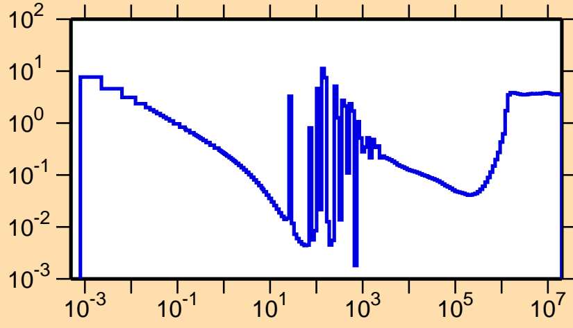
\sigma vs. E for ^{221}\text{Bi}(n,\text{nonel.})
