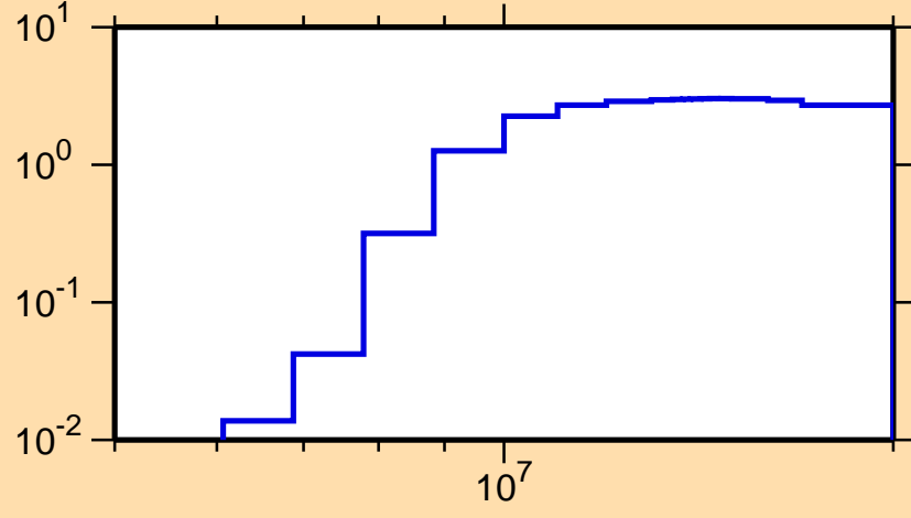
\sigma vs. E for ^{221}\text{Bi}(n,n\alpha)
