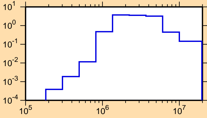
\sigma vs. E for ^{221}\text{Bi}(n,n\text{cont.})
