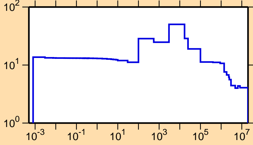
\sigma vs. E for ^{221}\text{Bi}(n,\text{el.})
