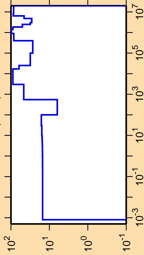
\Delta\sigma/\sigma vs. E for ^{221}\text{Bi}(n,\text{el.})
