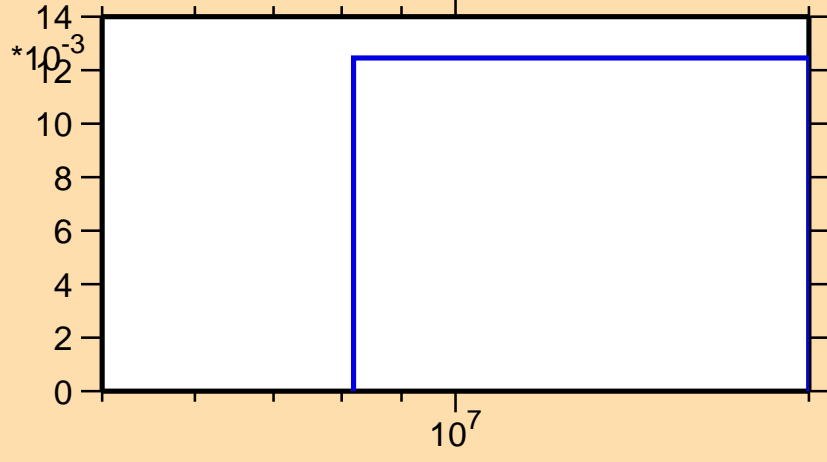
\sigma vs. E for ^{221}\text{Bi}(n,3n)
