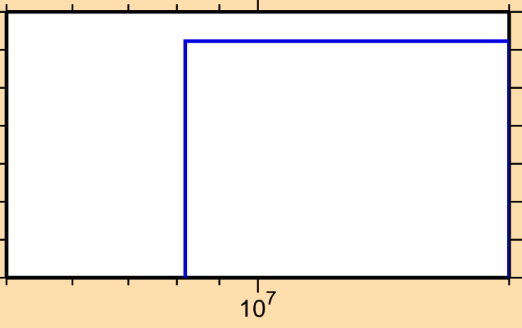
\sigma vs. E for ^{221}\text{Bi}(n,3n)
