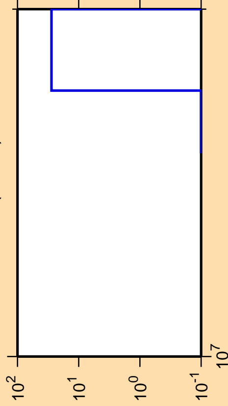
\Delta\sigma/\sigma vs. E for ^{222}\text{Bi} (mt 42)
