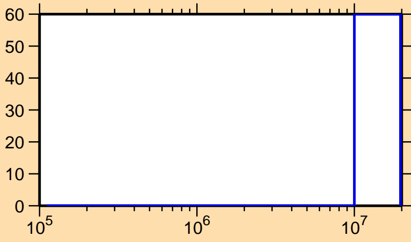
\Delta\sigma/\sigma vs. E for ^{222}\text{Bi}(n,f)
