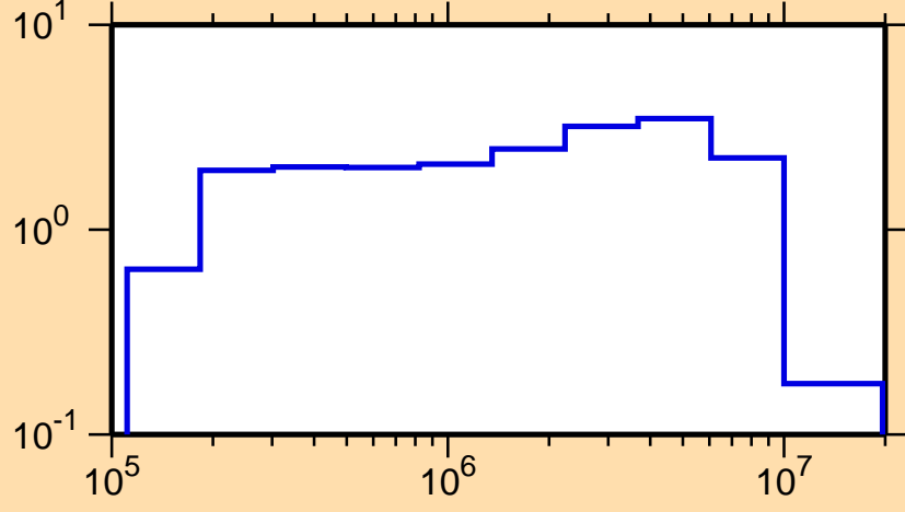
\sigma vs. E for ^{222}\text{Bi}(n,n\text{cont.})
