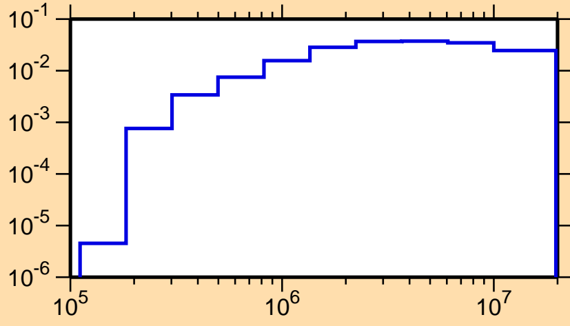
\sigma vs. E for ^{222}\text{Bi}(n,n_1)
