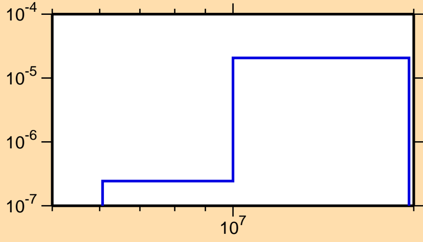
\sigma vs. E for ^{222}\text{Bi}(n,\alpha)
