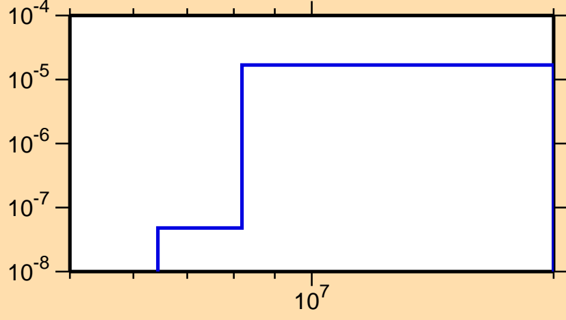
\sigma vs. E for ^{222}\text{Bi}(n,n\alpha)
