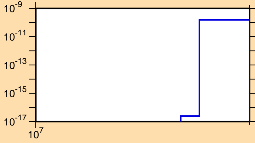
\sigma vs. E for ^{223}\text{Bi} (mt 11)
