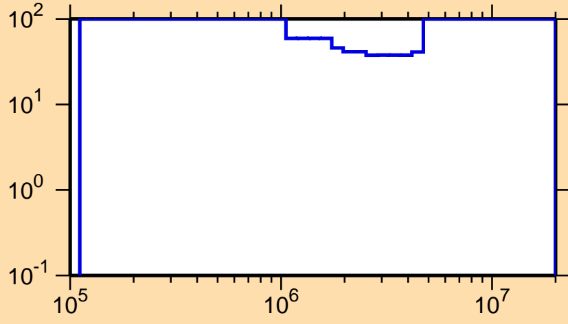
\Delta\sigma/\sigma vs. E for ^{223}\text{Bi}(n,inel.)
