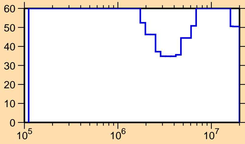
\Delta\sigma/\sigma vs. E for ^{223}\text{Bi}(n,\text{tot.})
