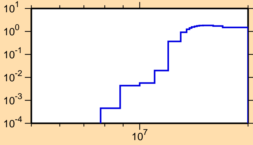
\sigma vs. E for ^{223}\text{Bi}(n,3n)
