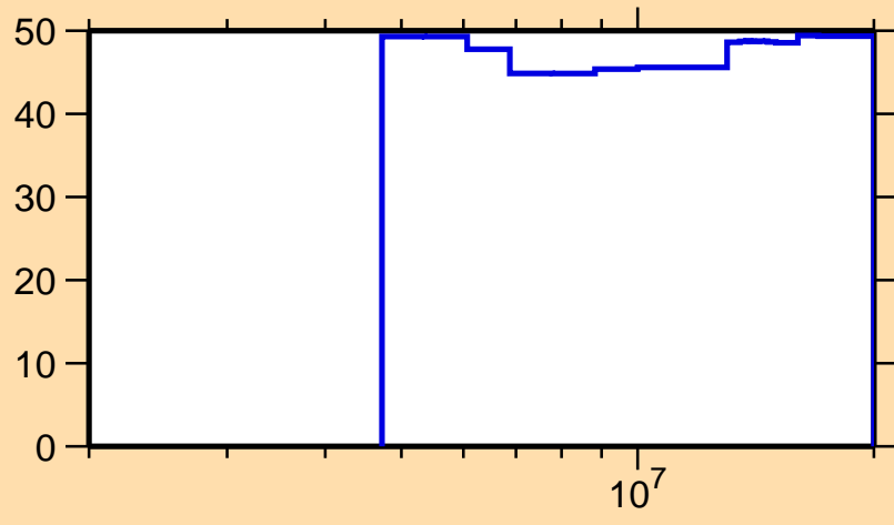
\Delta\sigma/\sigma vs. E for ^{223}\text{Bi}(n,\text{nonel.})
