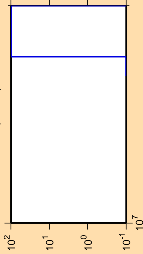
\Delta\sigma/\sigma vs. E for ^{223}\text{Bi} (mt 11)
