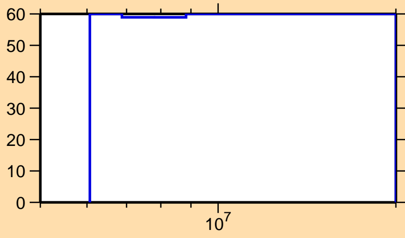
\Delta\sigma/\sigma vs. E for ^{223}\text{Bi}(n,2n)
