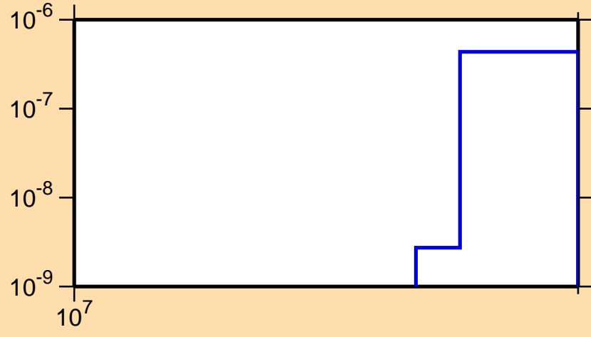
\sigma vs. E for ^{223}\text{Bi}(n,\text{nd})
