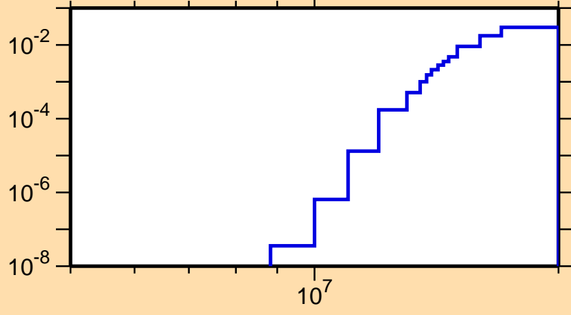
\sigma vs. E for ^{223}\text{Bi}(n,n\alpha)
