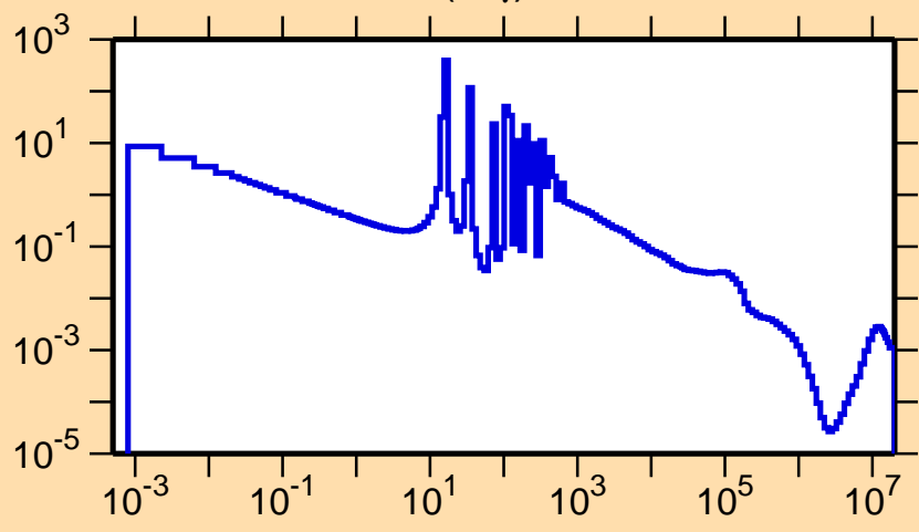
\sigma vs. E for ^{223}\text{Bi}(n,\gamma)
