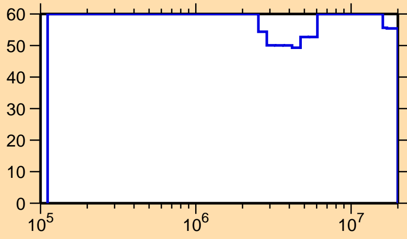
\Delta\sigma/\sigma vs. E for ^{223}\text{Bi}(n,\text{el.})
