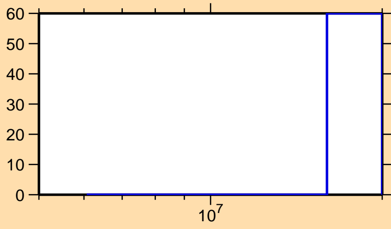
\Delta\sigma/\sigma vs. E for ^{223}\text{Bi}(n,f)
