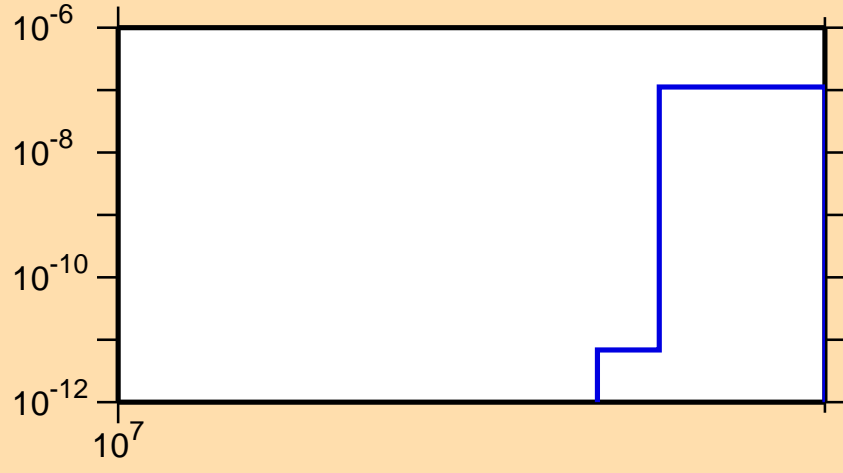
\sigma vs. E for ^{223}\text{Bi}(n,2np)
