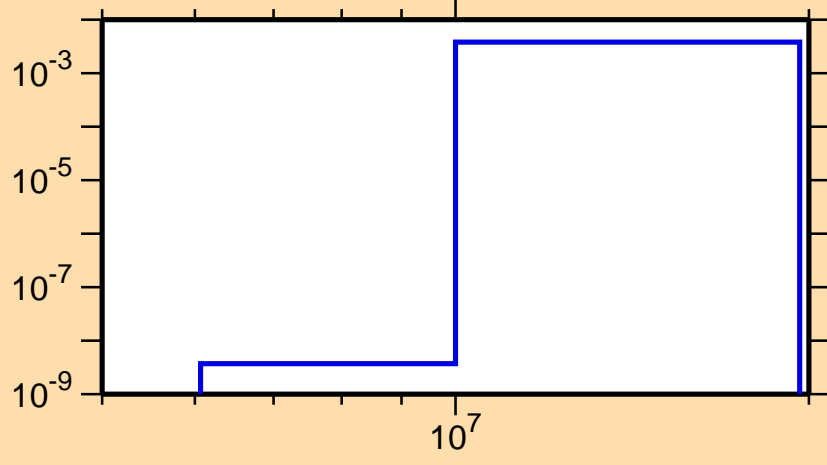
\sigma vs. E for ^{223}\text{Bi}(n,n\alpha)
