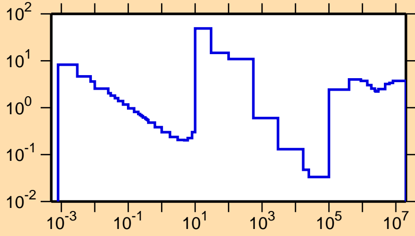
\sigma vs. E for ^{223}\text{Bi}(n,\text{nonel.})
