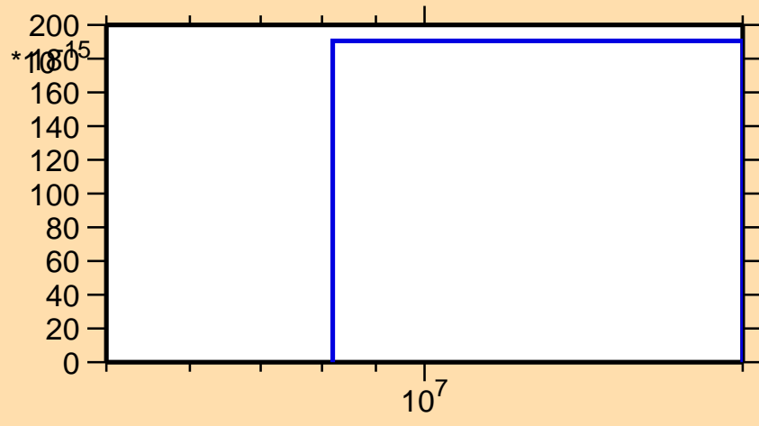
\sigma vs. E for ^{223}\text{Bi} (mt 42)
