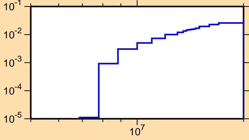
\sigma vs. E for ^{234}\text{Bk}(n,2n)
