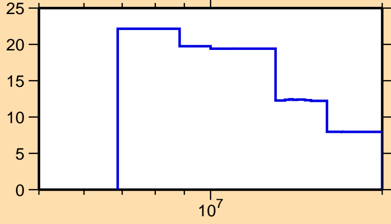
\Delta\sigma/\sigma vs. E for ^{234}\text{Bk}(n,\text{tot.})
