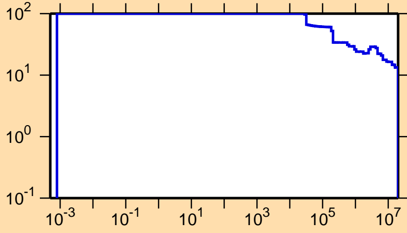
\Delta\sigma/\sigma vs. E for ^{234}\text{Bk}(n,\text{nonel.})
