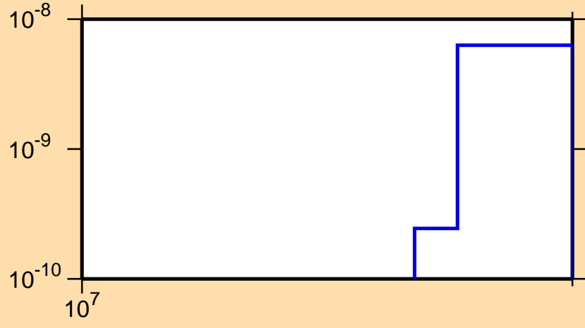
\sigma vs. E for ^{234}\text{Bk}(n,nt)
