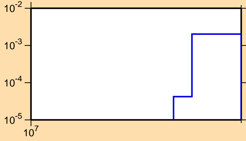
\sigma vs. E for ^{234}\text{Bk}(n,3n)
