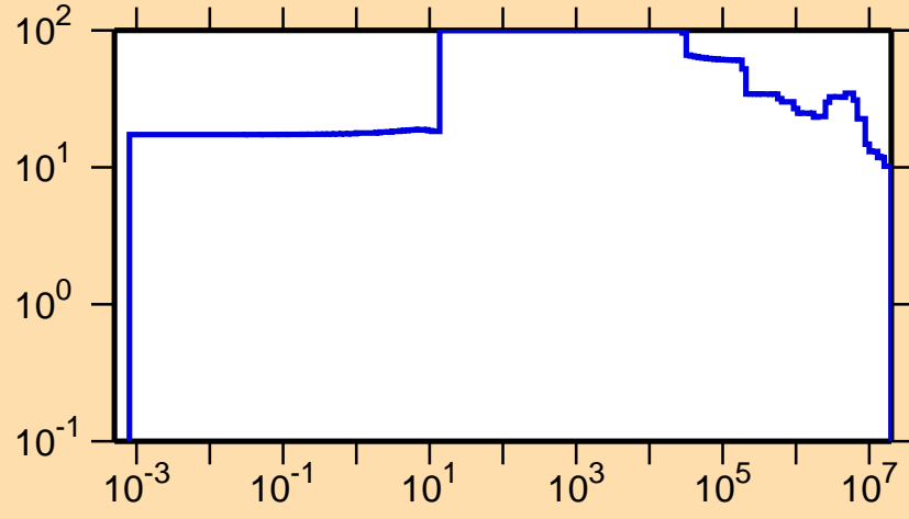
\Delta\sigma/\sigma vs. E for ^{234}\text{Bk}(n,f)
