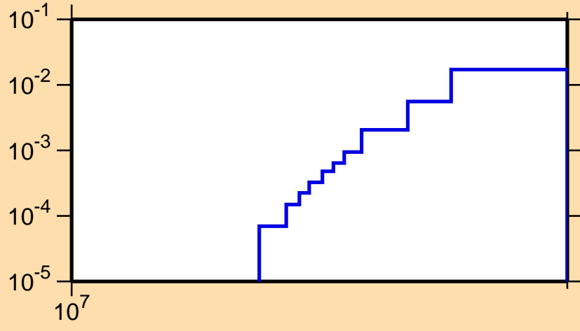
\sigma vs. E for ^{234}\text{Bk}(n,2np)
