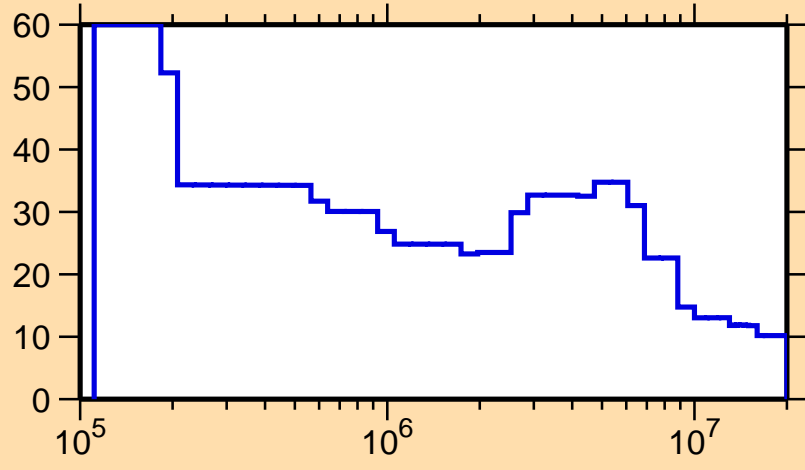
\Delta\sigma/\sigma vs. E for ^{234}\text{Bk}(n,f)
