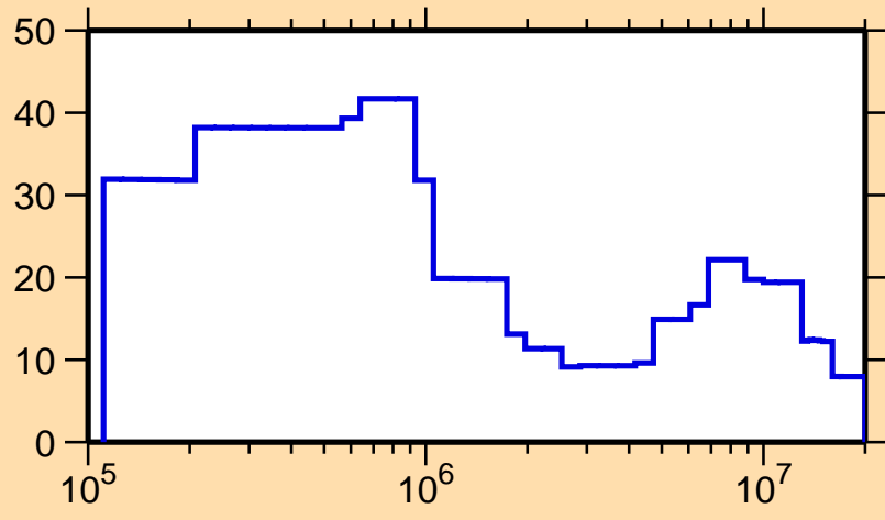
\Delta\sigma/\sigma vs. E for ^{234}\text{Bk}(n,\text{tot.})
