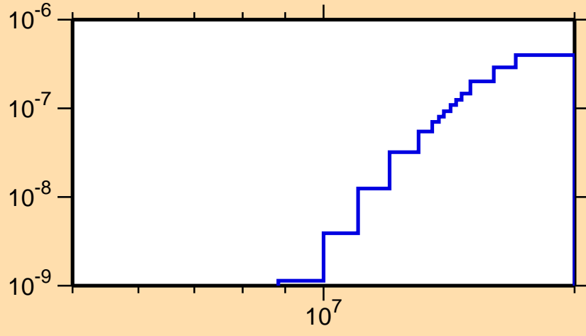
\sigma vs. E for ^{234}\text{Bk}(n,p\alpha)
