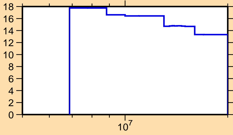
\Delta\sigma/\sigma vs. E for ^{234}\text{Bk}(n,\text{nonel.})
