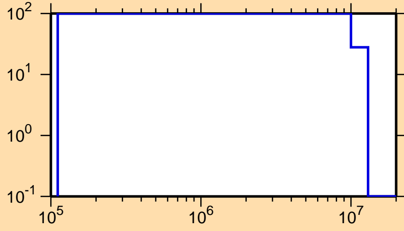
\Delta\sigma/\sigma vs. E for ^{234}\text{Bk}(n,n_1)
