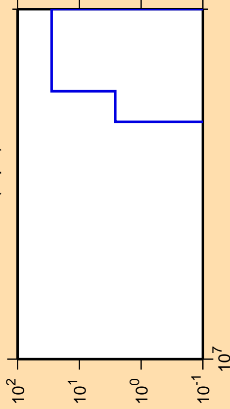
\Delta\sigma/\sigma vs. E for ^{234}\text{Bk}(n,pd)
