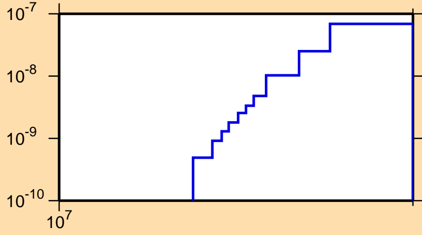
\sigma vs. E for ^{234}\text{Bk}(n,nd)
