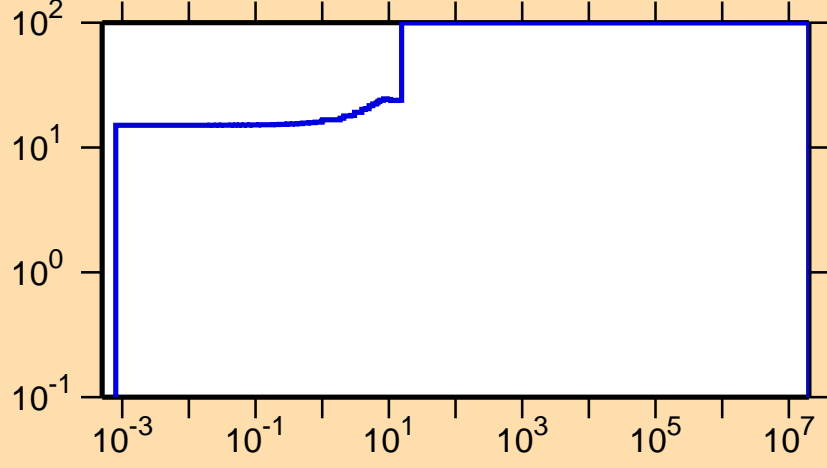
\Delta\sigma/\sigma vs. E for ^{234}\text{Bk}(n,\gamma)
