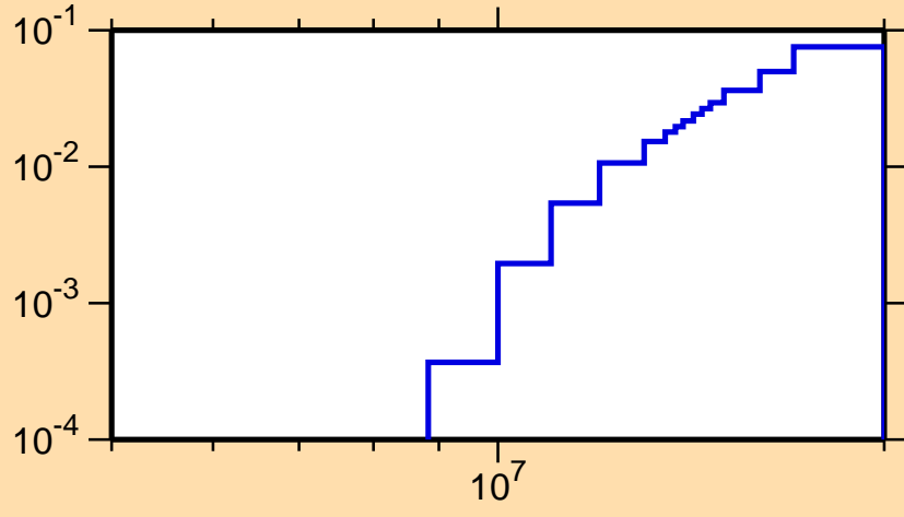
\sigma vs. E for ^{234}\text{Bk}(n,2n\alpha)
