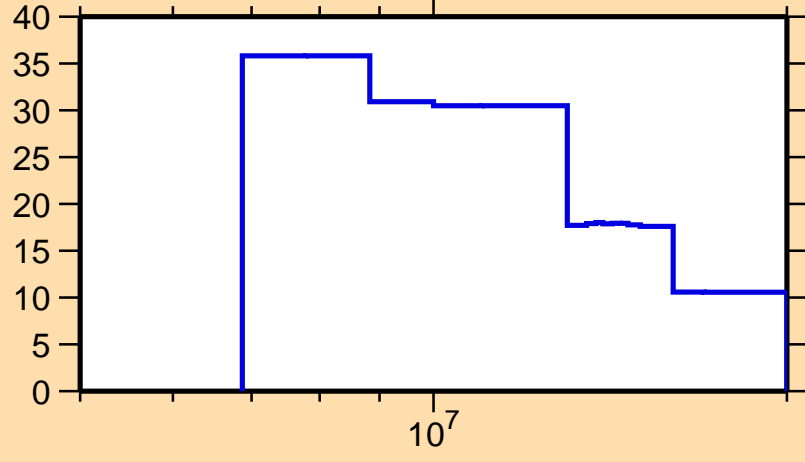
\Delta\sigma/\sigma vs. E for ^{234}\text{Bk}(n,\text{el.})
