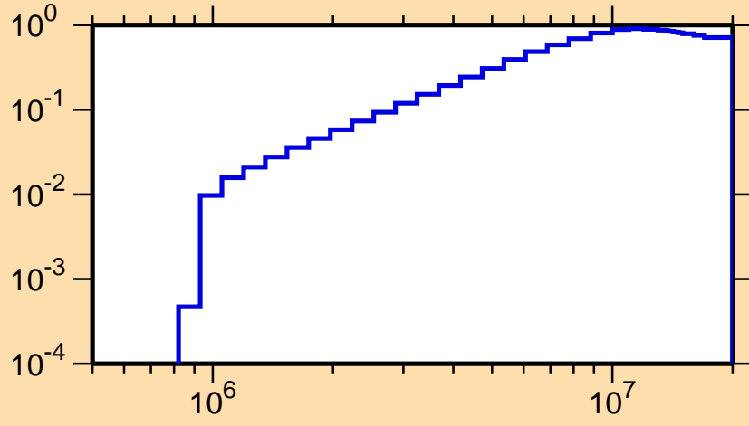
\sigma vs. E for ^{234}\text{Bk}(n,\text{inel.})
