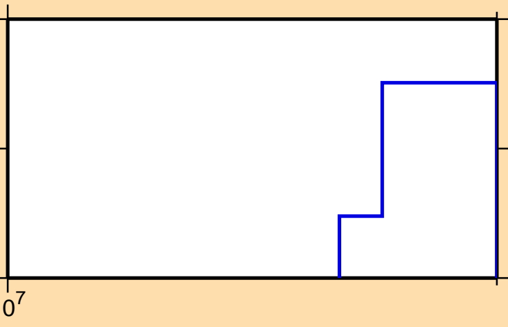
\sigma vs. E for ^{234}\text{Bk}(n,pd)
