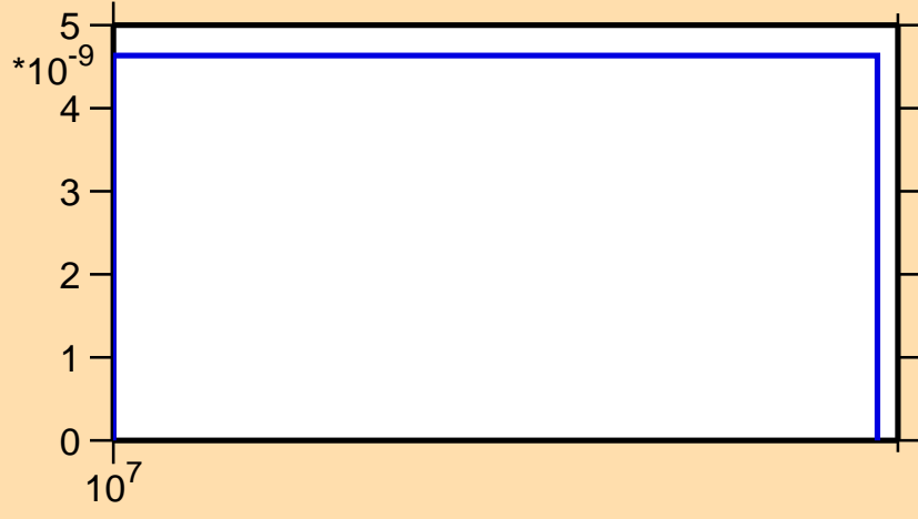
\sigma vs. E for ^{234}\text{Bk}(n,\text{nd})
