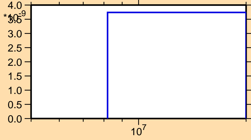
\sigma vs. E for ^{234}\text{Bk}(n,nd)
