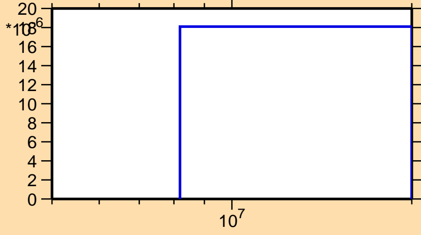
\sigma vs. E for ^{234}\text{Bk}(n,3n)
