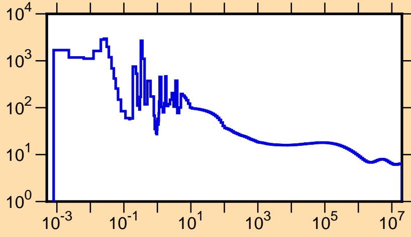
\sigma vs. E for ^{237}\text{Bk}(n,\text{tot.})
