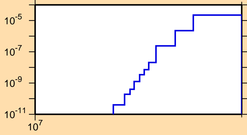
\sigma vs. E for ^{237}\text{Bk}(n,\text{nd})
