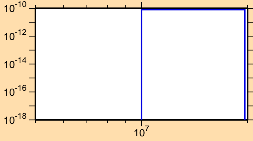
\sigma vs. E for ^{237}\text{Bk}(n,2n\alpha)
