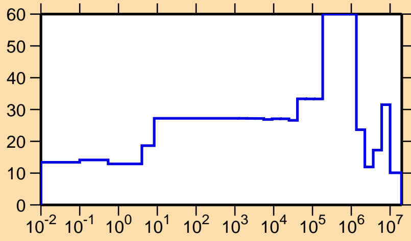
\Delta\sigma/\sigma vs. E for ^{237}\text{Bk}(n,el.)
