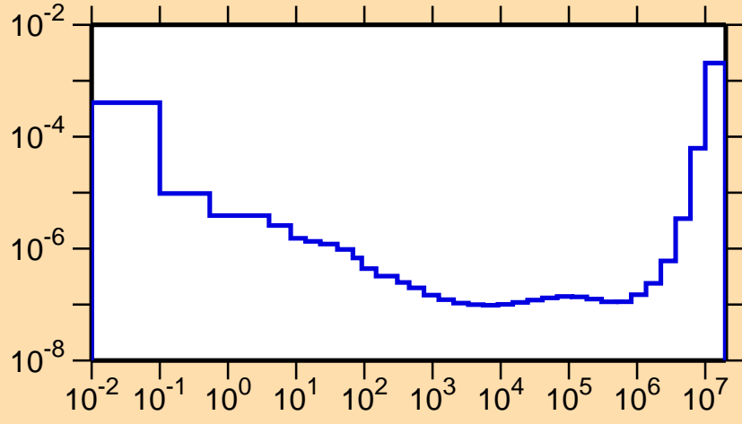
\sigma vs. E for ^{237}\text{Bk}(n,\alpha)
