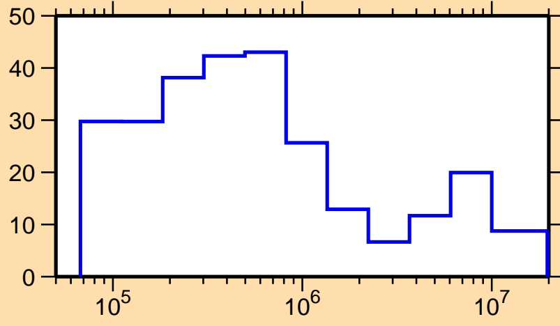
\Delta\sigma/\sigma vs. E for ^{237}\text{Bk}(n,tot.)
