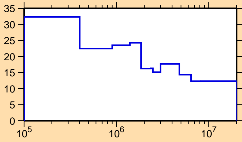
\Delta\sigma/\sigma vs. E for ^{237}\text{Bk}(n,\text{nonel.})
