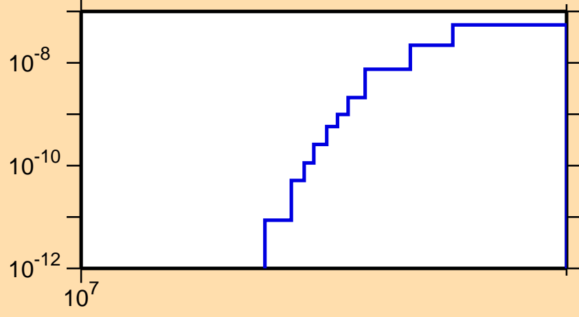
\sigma vs. E for ^{238}\text{Bk}(n,2np)
