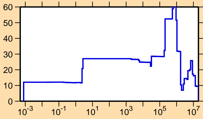
\Delta\sigma/\sigma vs. E for ^{238}\text{Bk}(n,el.)
