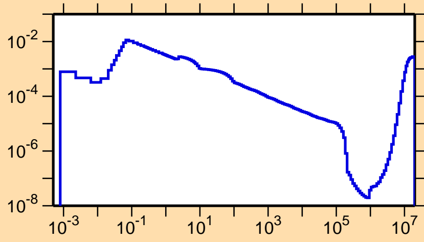
\sigma vs. E for ^{238}\text{Bk}(n,\alpha)
