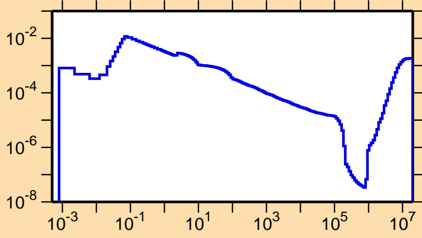
\sigma vs. E for ^{238}\text{Bk}(n,p)
