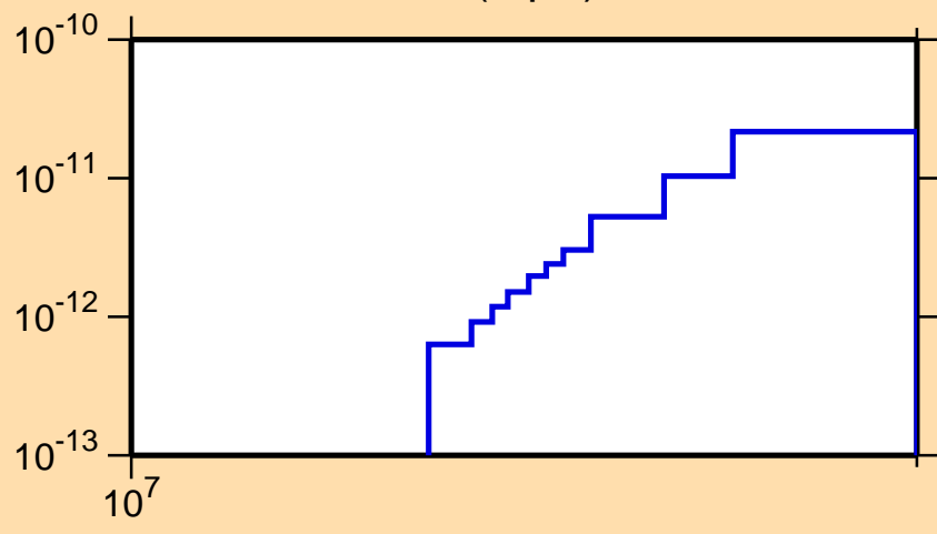
\sigma vs. E for ^{238}\text{Bk}(n,p\alpha)
