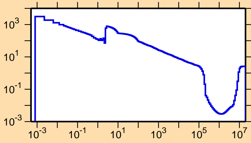
\sigma vs. E for ^{238}\text{Bk}(n,f)
