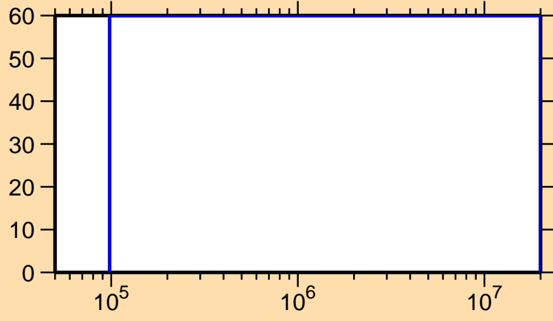
\Delta\sigma/\sigma vs. E for ^{238}\text{Bk}(n,n\text{cont.})
