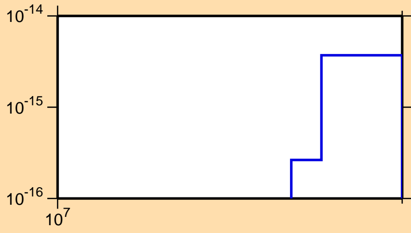
\sigma vs. E for ^{238}\text{Bk} (mt 34)
