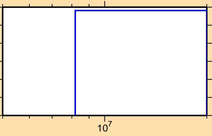
\sigma vs. E for ^{238}\text{Bk}(n,\text{He3})
