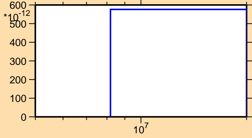
\sigma vs. E for ^{238}\text{Bk}(n,\text{nd})
