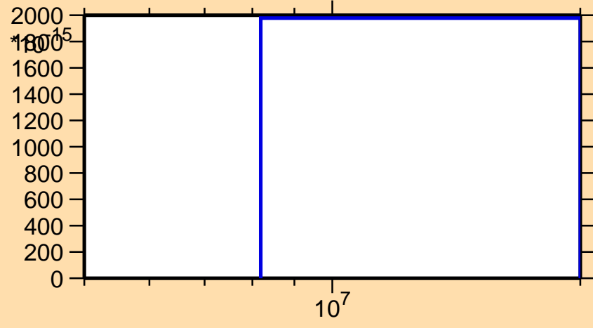
\sigma vs. E for ^{238}\text{Bk}(n,p\alpha)
