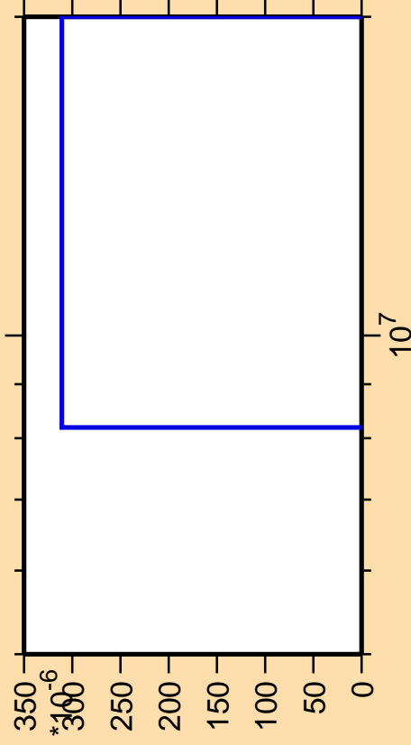
\Delta\sigma/\sigma vs. E for ^{238}\text{Bk}(\text{mt } 34)
