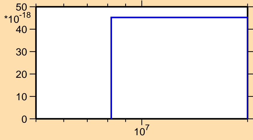
\sigma vs. E for ^{238}\text{Bk}(\text{mt } 34)
