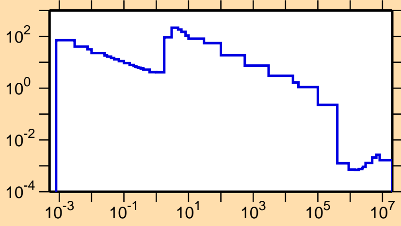
\sigma vs. E for ^{238}\text{Bk}(n,\gamma)
