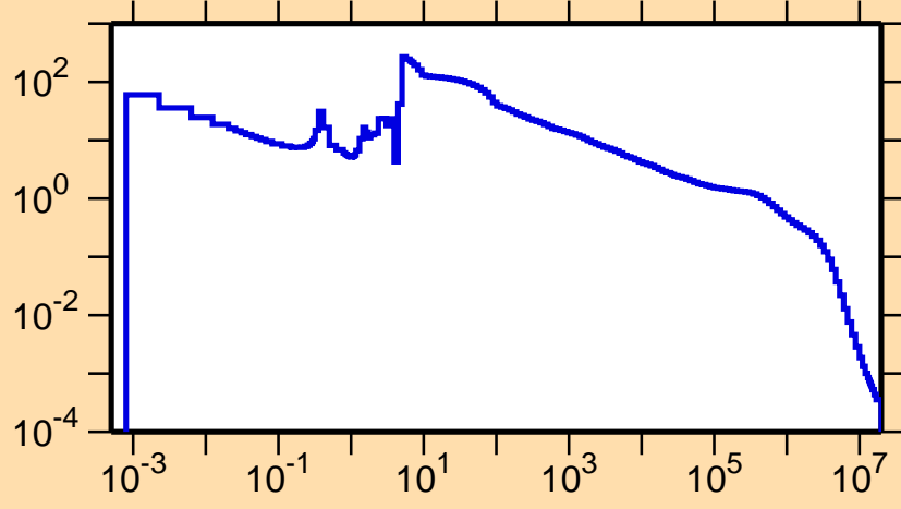
\sigma vs. E for ^{240}\text{Bk}(n,\gamma)
